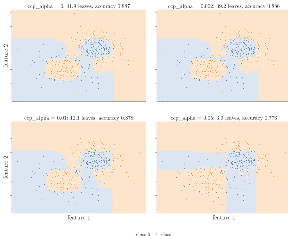
Figure 4: Forests of 100 trees pruned with four values of ccp_alpha ; titles give the leaves per tree and the mean test accuracy over 20 splits
