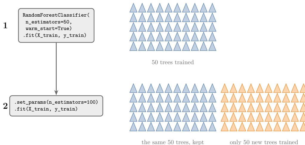
Figure 5: warm_start in two steps: the first fit trains 50 trees; after set_params(n_estimators=100) , the second fit keeps those 50 and trains only 50 new ones
