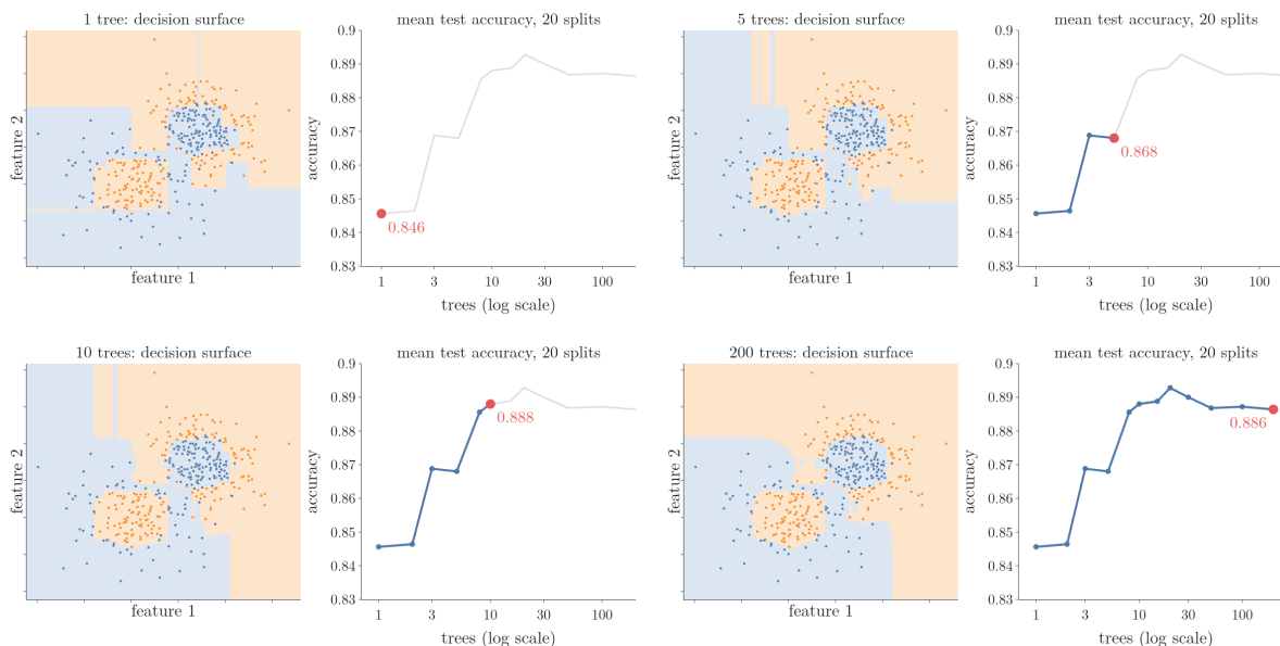
Figure 3: The forest grows from 1 to 200 trees. Left: the decision surface on one split. Right: the mean test accuracy over 20 splits, drawn up to the current number of trees (log scale)
