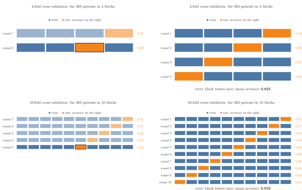
Figure 3: Cross-validation as rotating blocks on the heart data: each round trains the default random forest on the blue blocks and tests it on the orange one; first 4 folds, then 10. Idea after StatQuest, “Machine Learning Fundamentals: Cross Validation”
