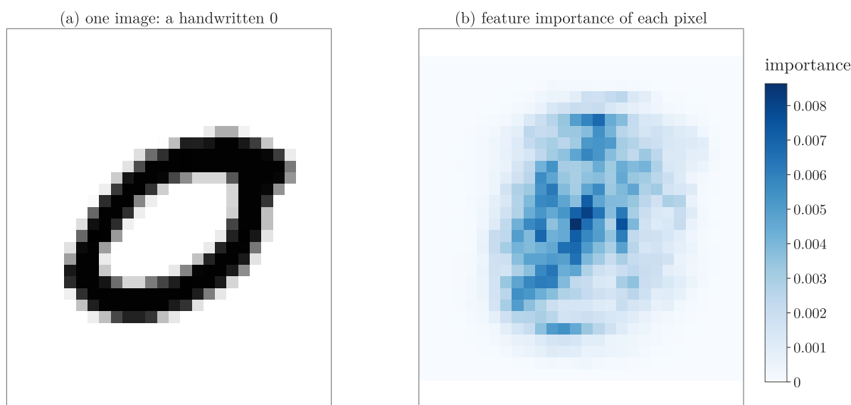
Figure 1: MNIST: (a) one handwritten digit; (b) the random forest's feature importance of each of the 784 pixels. Darker means more important. A heatmap shows each number of a grid as a colour
