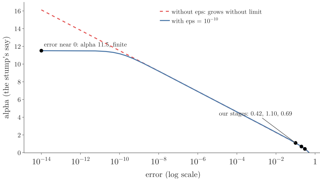
Figure 6: Alpha against the error on a log scale. Without eps (dashed) alpha grows without limit as the error falls to 0; with \text{eps} = 10^{-10} it levels off at 11.5. Our three stages sit at the far right
