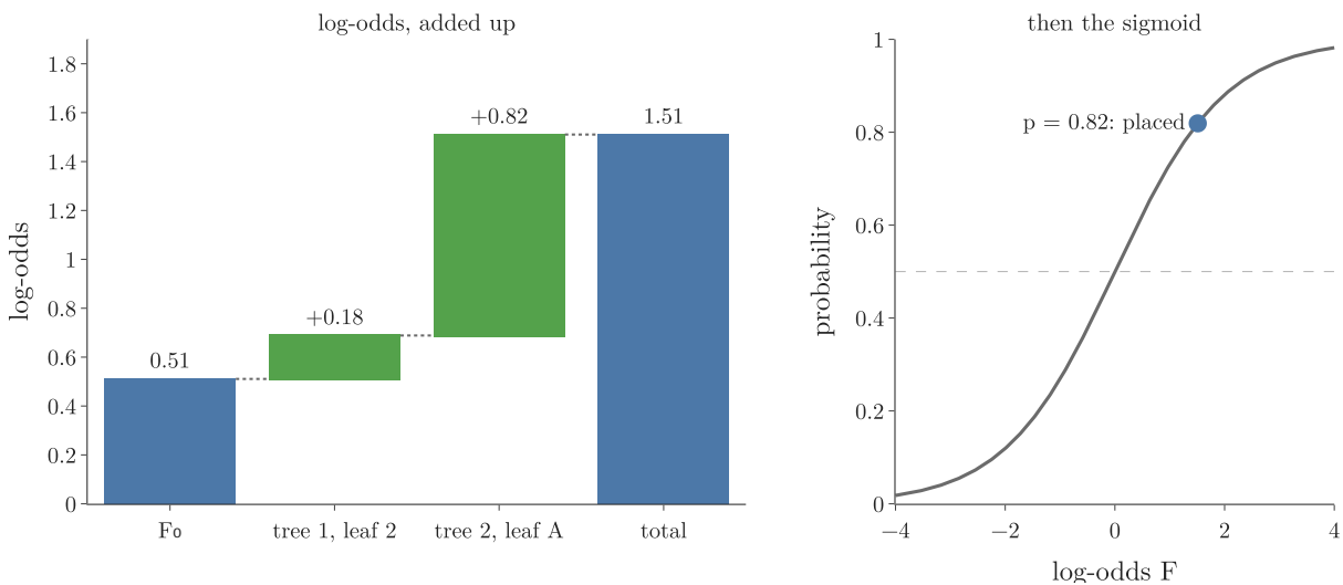
Figure 9: The new student (CGPA 7.2, IQ 100): F_0 = 0.51 plus 0.18 from tree 1 and 0.82 from tree 2 gives log-odds 1.51 (left); the sigmoid turns it into probability 0.82 (right)
