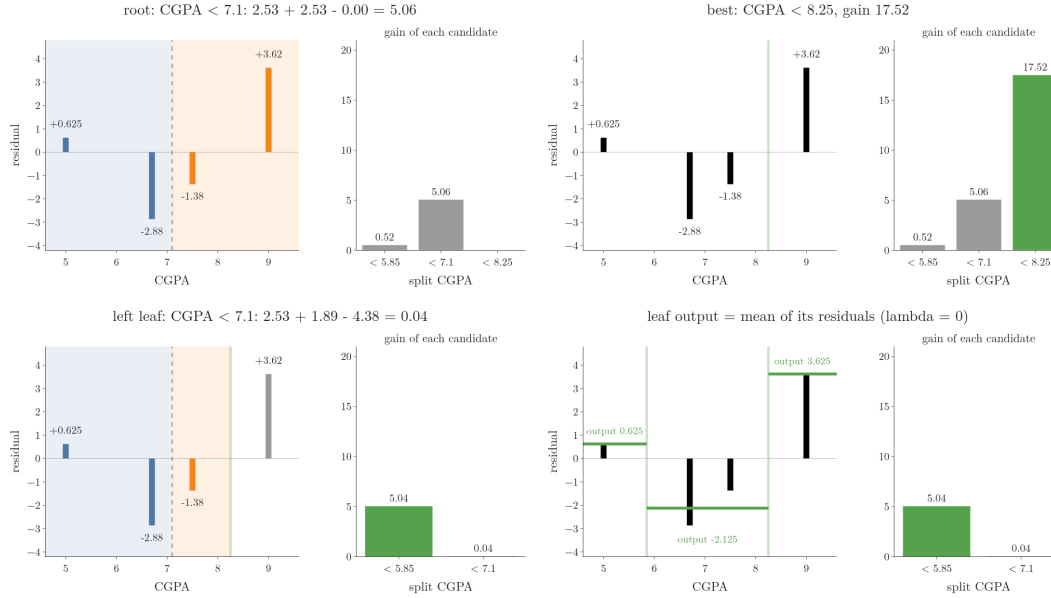
Figure 5: The XGBoost split search on the four students (lambda = 0). Left: the residuals, the sliding threshold and the locked splits (green). Right: the gain of each candidate, S_{\text{left}} + S_{\text{right}} - S_{\text{parent}} . Last frame: the outputs of the three leaves. The sliding-threshold picture follows StatQuest’s “XGBoost Part 1: Regression” (Starmer)
