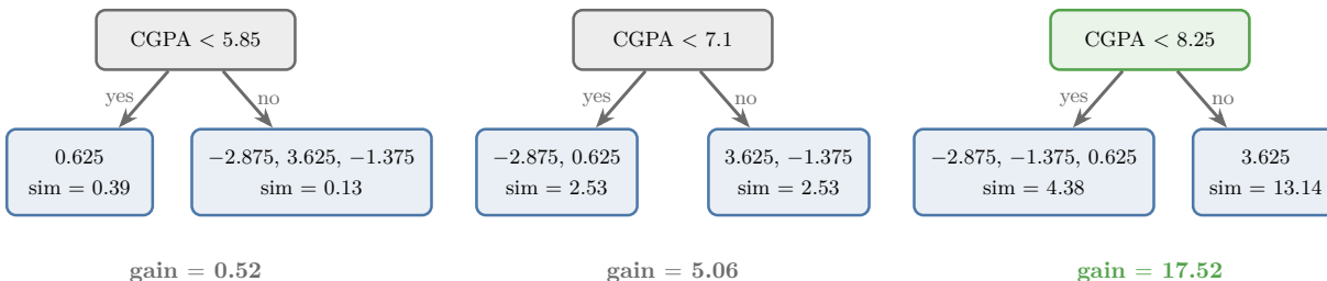
Figure 4: The three candidate root splits, with each leaf's residuals and similarity score; \text{CGPA} < 8.25 has by far the largest gain
