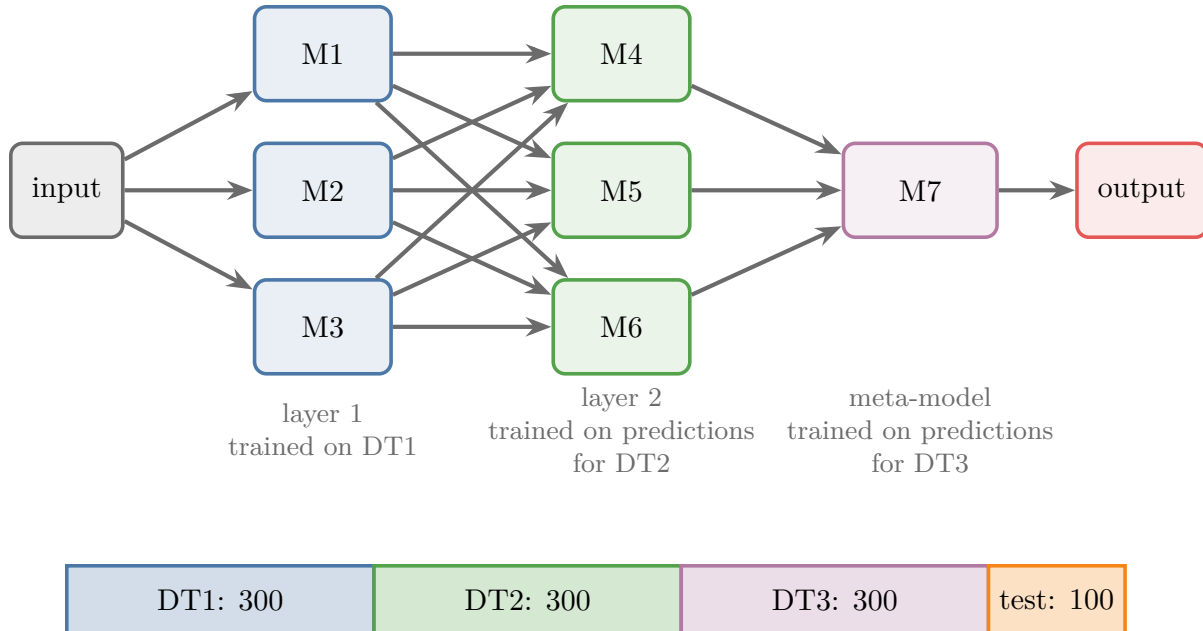
Figure 7: Two layers of base models and a meta-model, trained with blending on three hold-out sets of 300 observations
