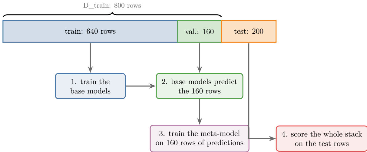
Figure 4: Blending: 1,000 observations split into 800 for training and 200 for testing; the 800 are split again into 640 for the base models and 160 for the meta-model
