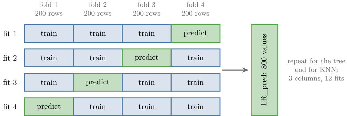
Figure 5: K-fold stacking with K = 4 : each fit trains on three folds and predicts the fourth; the four predicted folds together fill one column of 800 out-of-fold predictions
