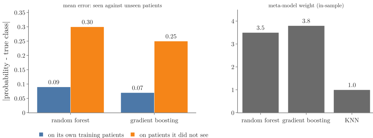
Figure 3: The leak in numbers on the heart data. Left: the random forest and gradient boosting look three times better on their own training patients than on unseen ones. Right: the meta-model trained on those in-sample predictions trusts them most
