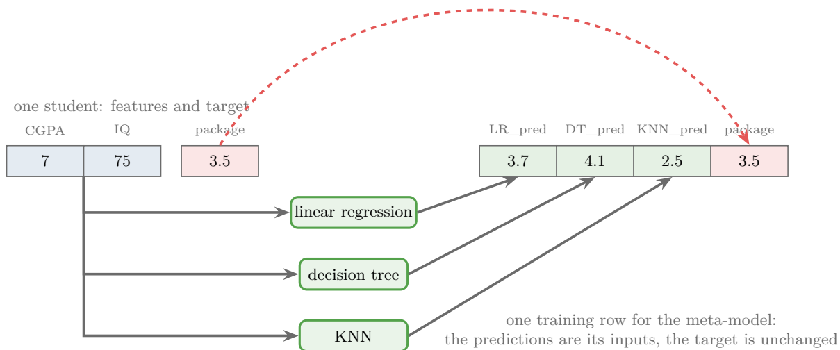
Figure 2: One student becomes one training row for the meta-model. The features go into the three base models; their predictions 3.7, 4.1 and 2.5 are the new row's inputs, and the target 3.5 stays the same
