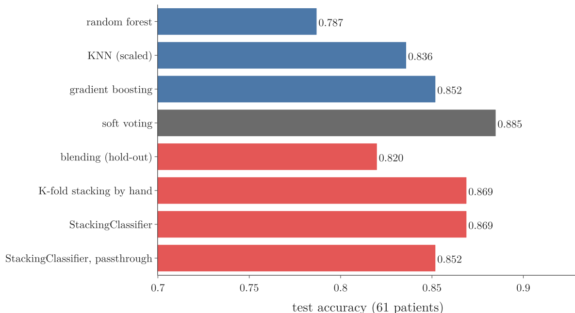
Figure 8: Test accuracy of the base models alone, soft voting and four kinds of stacking on the heart data (KNN scaled)
