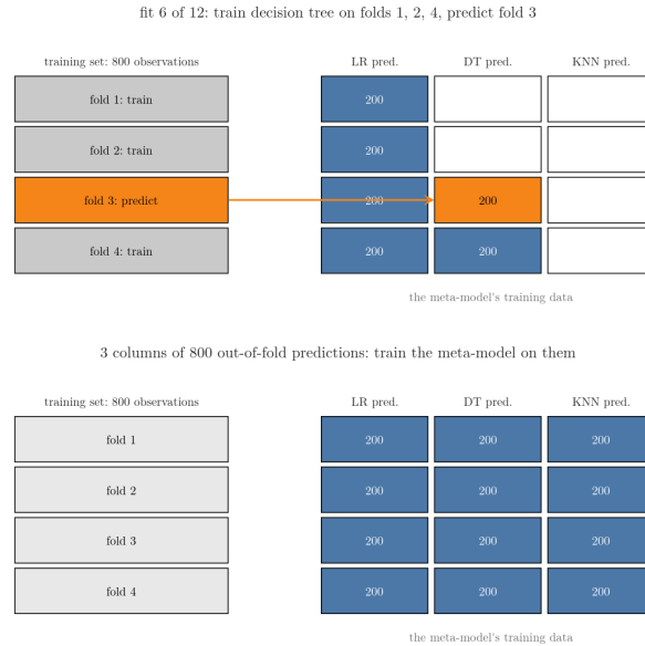
Figure 6: K-fold stacking with K = 4 , one fit per frame. Left: the four folds of the training set; grey folds train the base model, the orange fold is predicted. Right: the meta-model's training data, one column of out-of-fold predictions per base model, filling 200 observations at a time.
