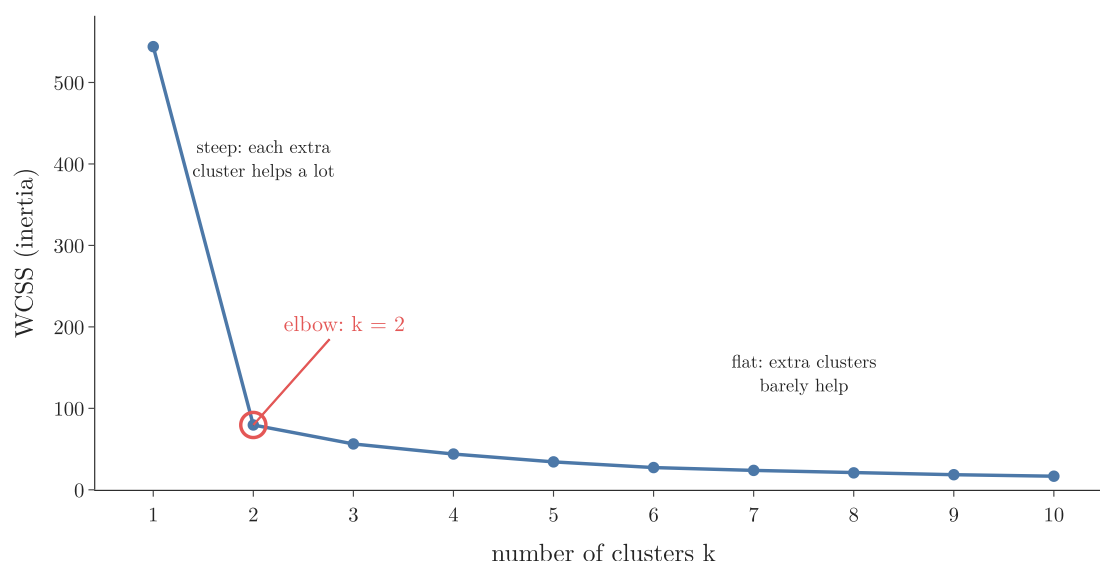
Figure 5: Elbow curve: WCSS against k for the 272 Old Faithful eruptions (standardized); the curve bends at k = 2
