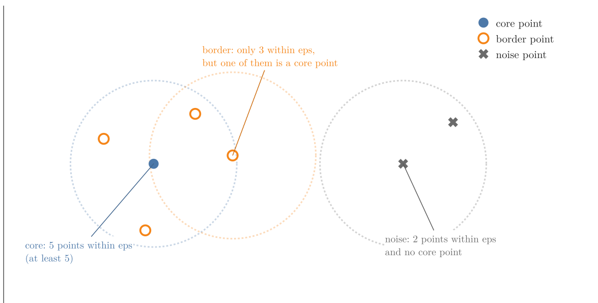
Figure 4: Core, border and noise points for \epsilon = 1 and MinPts = 5; dotted circles are \epsilon -neighbourhoods
