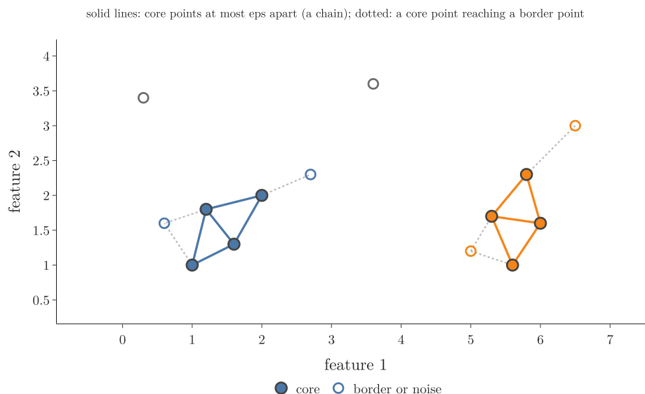
Figure 5: Density-connected points. Solid lines join core points at most \text{eps} apart; dotted lines join a core point to a border point, which ends a chain. Each chain of core points is one cluster (blue, orange); the two grey points are noise
