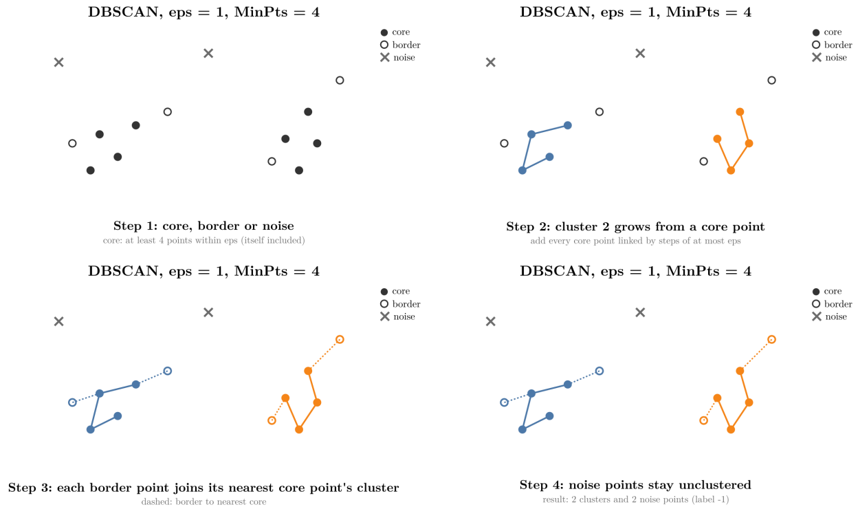
Figure 6: DBSCAN step by step: label points, grow clusters through core points, attach border points, leave noise
