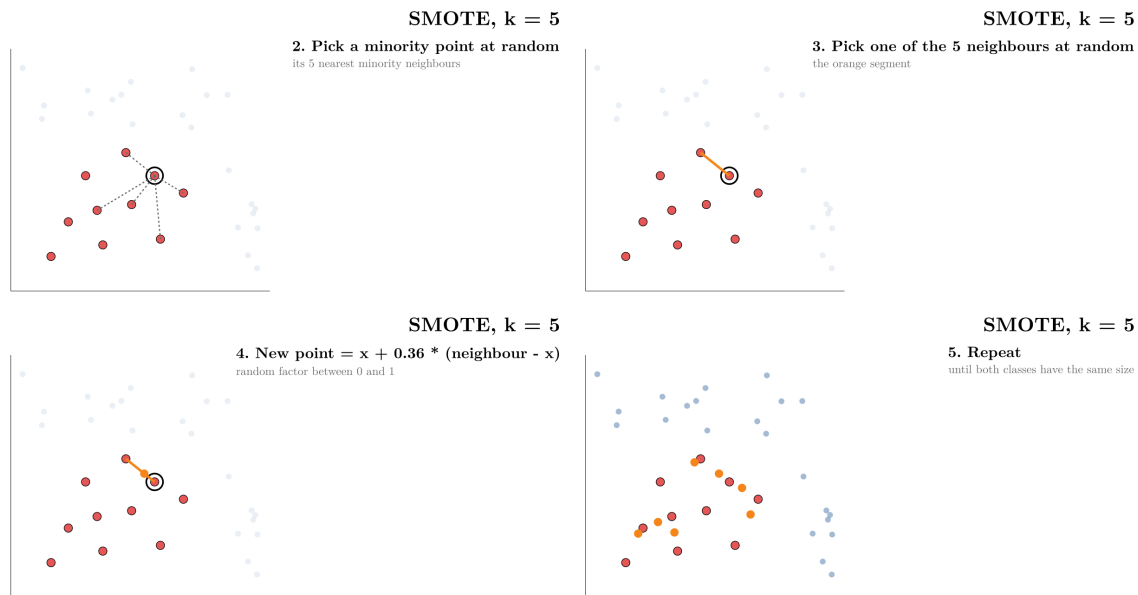
Figure 7: SMOTE step by step: a random minority point and its 5 nearest minority neighbours, one neighbour chosen, a new point between them, and the result after a few repetitions
