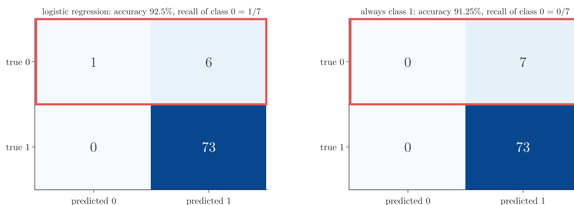
Figure 4: Confusion matrices on the 80 test observations. Left: logistic regression finds 1 of the 7 minority observations (red row). Right: a model that always answers class 1 finds none, and still scores 91.25%
