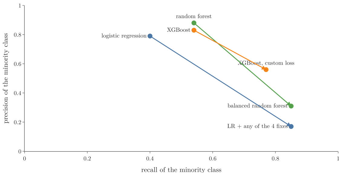
Figure 12: Minority precision against minority recall on the mammography data. Each arrow goes from a model as is to the same model with a fix: every fix moves right (more calcifications found) and down (more false alarms)
