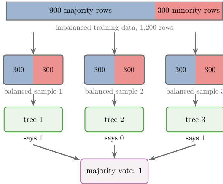
Figure 10: A balanced random forest: every tree is trained on a balanced sample, then the trees vote
