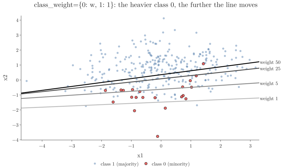
Figure 11: The line logistic regression learns as the weight of class 0 grows from 1 to 50
