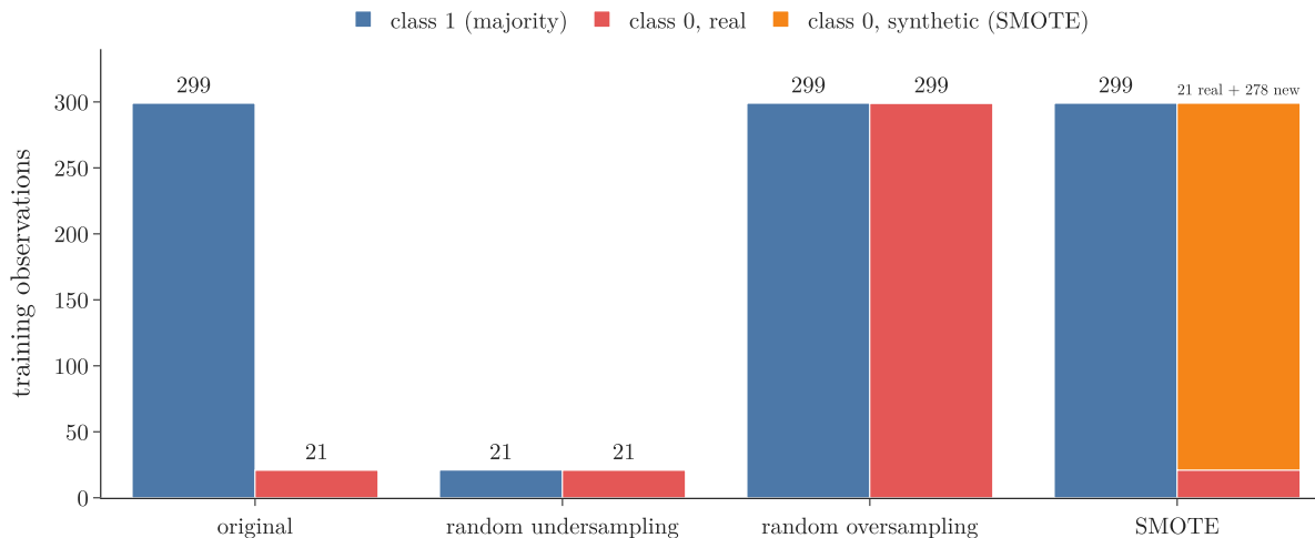
Figure 6: The training set’s class counts before and after each resampler. Undersampling cuts the majority to 21; oversampling copies the minority up to 299; SMOTE adds 278 new minority points
