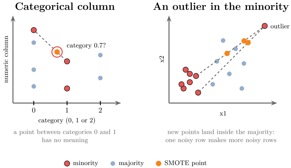
Figure 8: Two SMOTE failures: a new point between two categories, and an outlier that spreads new points into the majority
