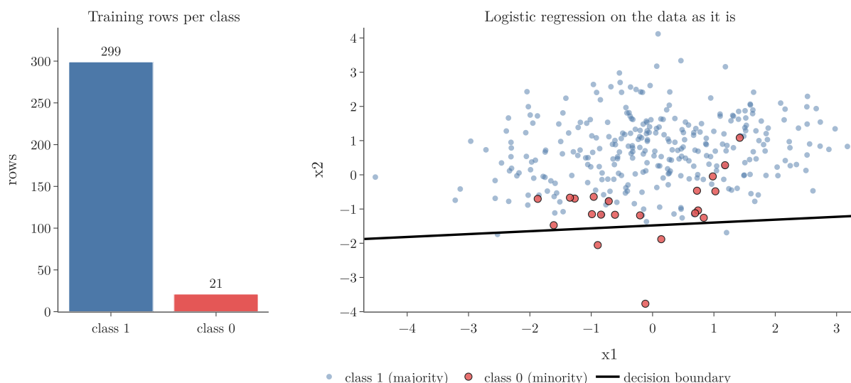
Figure 3: Left: the training observations per class. Right: the line logistic regression learns on this data
