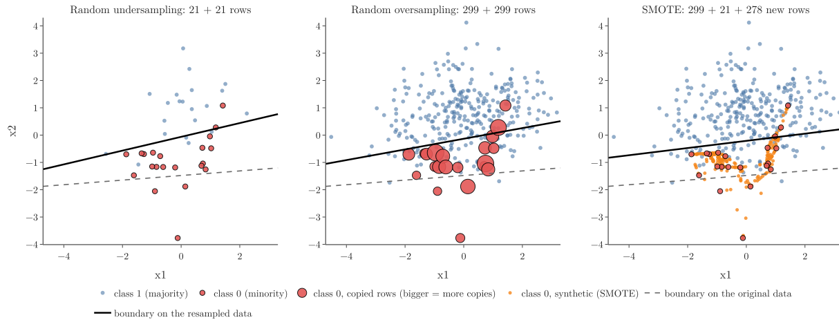
Figure 5: The training data after random undersampling, random oversampling and SMOTE. Solid line: logistic regression trained on the resampled data; dashed line: trained on the original data
