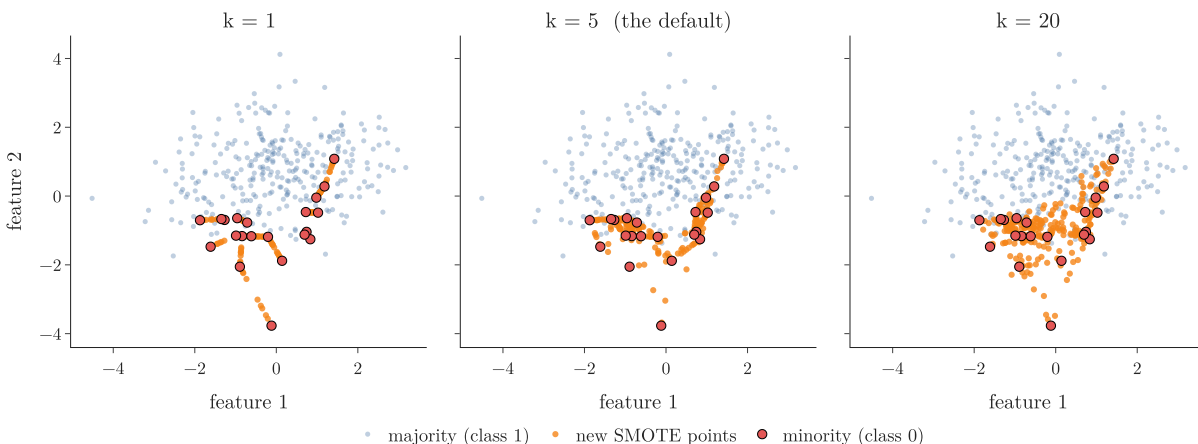
Figure 9: The 278 new SMOTE points (orange) on our training data for k = 1 , 5 and 20. With k = 1 the new points line up on a few short segments; with k = 20 almost every minority point is a neighbour of every other, and the new points spread over the area between them, into the majority.
