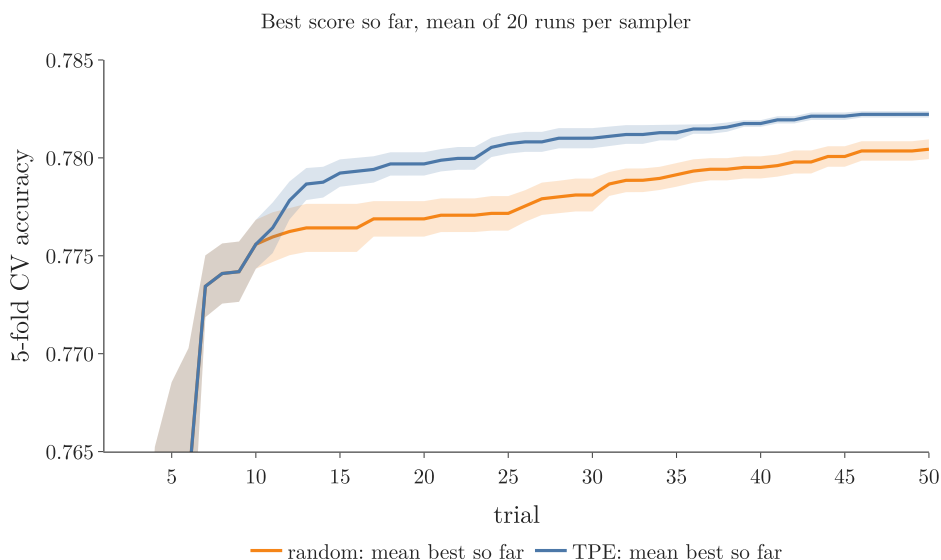
Figure 6: Best 5-fold CV accuracy so far, averaged over 20 runs of each sampler on the SVM search; the bands are \pm one standard error
