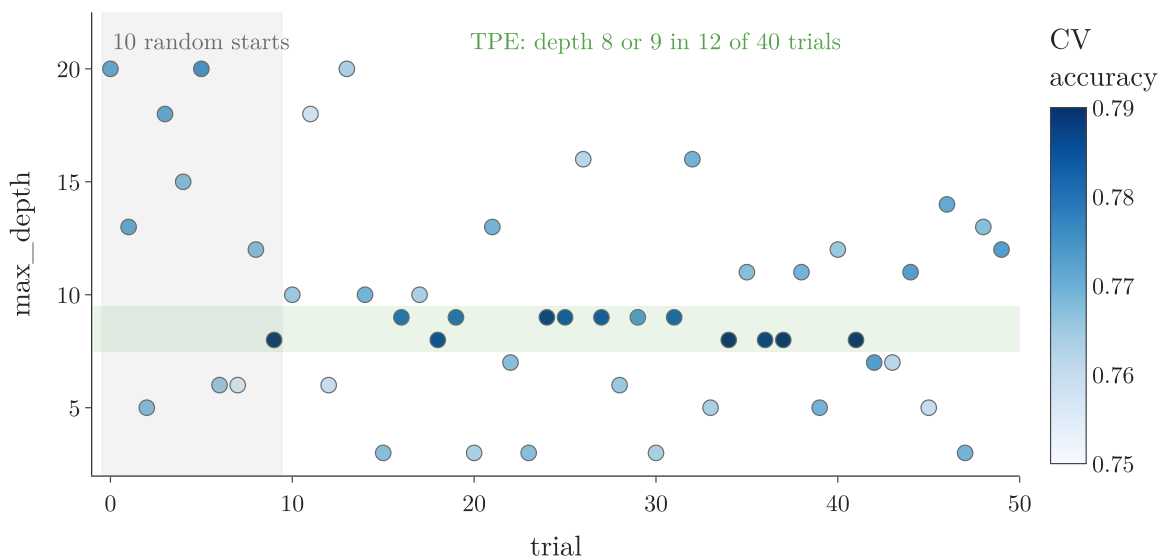
Figure 4: The TPE study's max_depth , trial by trial: random for 10 trials, then returning again and again to depth 8 and 9 (green band); darker dots scored higher
