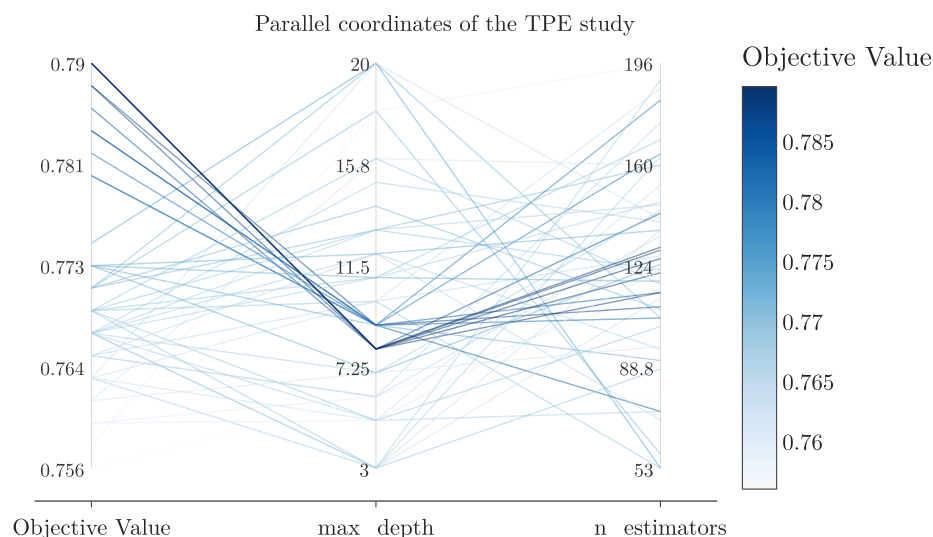
Figure 8: Parallel coordinates of the TPE study: each line is a trial, darker is a higher score
