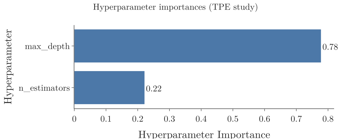
Figure 11: Hyperparameter importances of the TPE study
