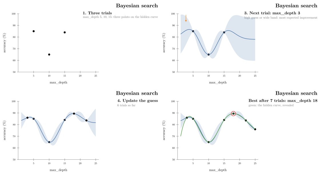
Figure 3: Bayesian search on one hyperparameter: three trials, a guess of the curve with its uncertainty (band), the next trial where the improvement could be largest, and the hidden curve revealed at the end
