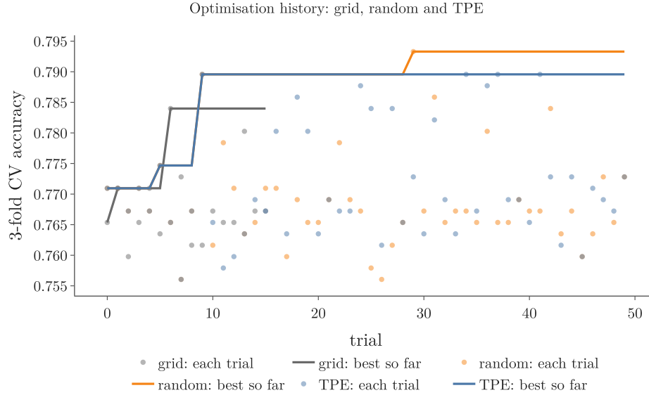
Figure 7: Optimisation history of the three studies: each trial (dots) and the best so far (lines)
