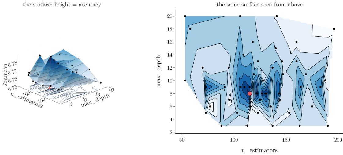
Figure 9: The accuracy surface of the TPE study (left) and the same surface seen from above (right). Black dots: the 50 trials. Red dot: the best trial.
