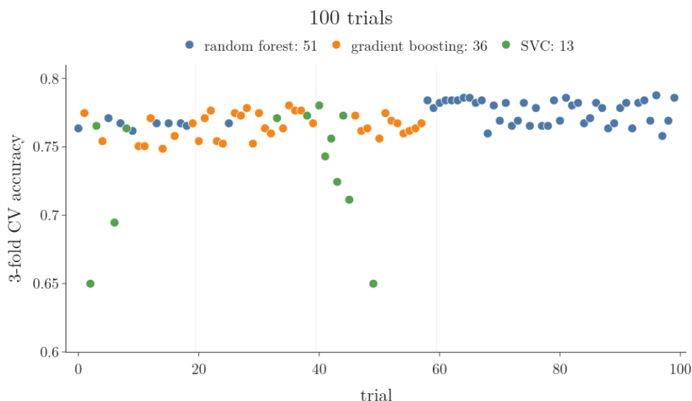
Figure 12: The define-by-run study, 5 trials per frame: each dot is a trial, coloured by its classifier
