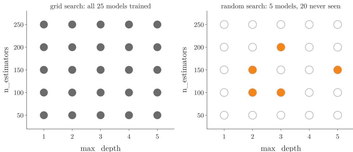
Figure 2: The 5 \times 5 placement grid: grid search trains all 25 combinations (left), random search 5 of them (right)
