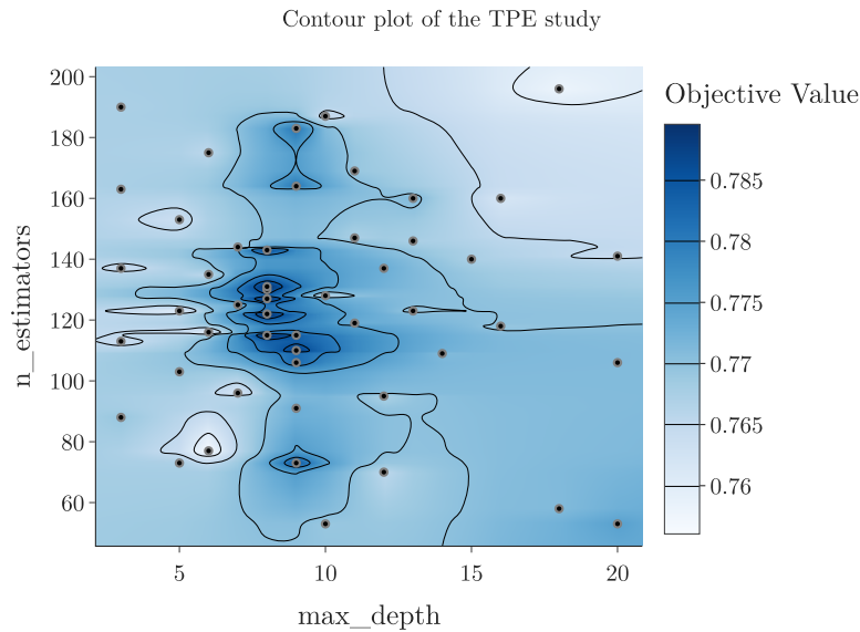
Figure 10: Contour plot of the TPE study: max_depth against n_estimators , darker is a higher score; dots are trials
