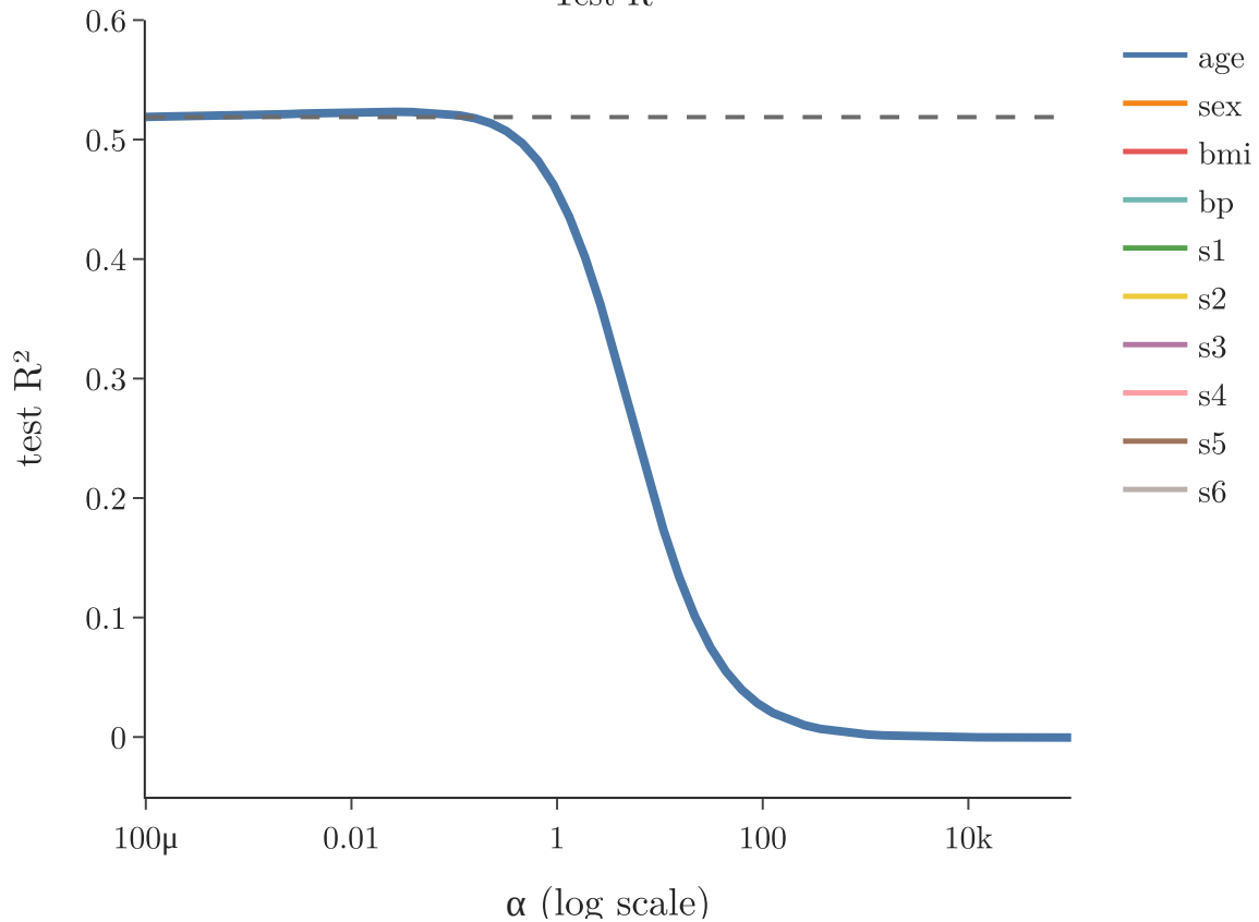
Test R^2
