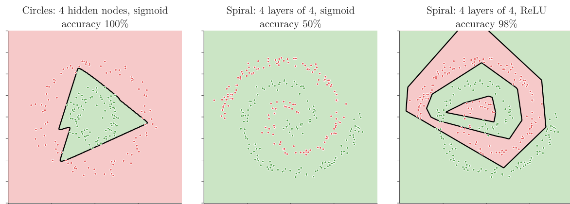
Figure 10: MLPs trained on two circles and on two spirals
