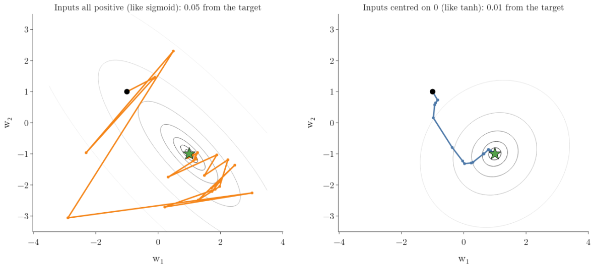
Figure 3: Stochastic gradient descent on one node with two weights. Left: inputs all positive. Right: the same inputs centred on 0. Grey: contours of the loss; black dot: start; star: the target weights.
