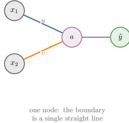
Figure 2: (a) After a start where all weights are equal, every weight leaving x_1 has one value u and every weight leaving x_2 one value v , so the hidden nodes all compute the same a . (b) The network behaves like a single hidden node
