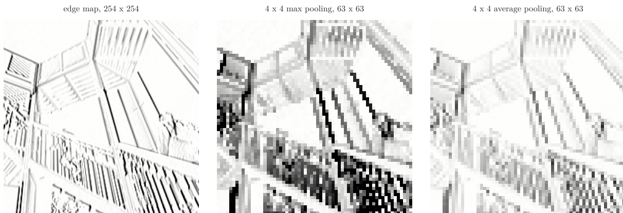
Figure 7: The vertical-edge map of a photo (left), after 4 \times 4 max pooling (middle) and after 4 \times 4 average pooling (right), on the same colour scale. Max pooling keeps the edges strong; averaging fades them
