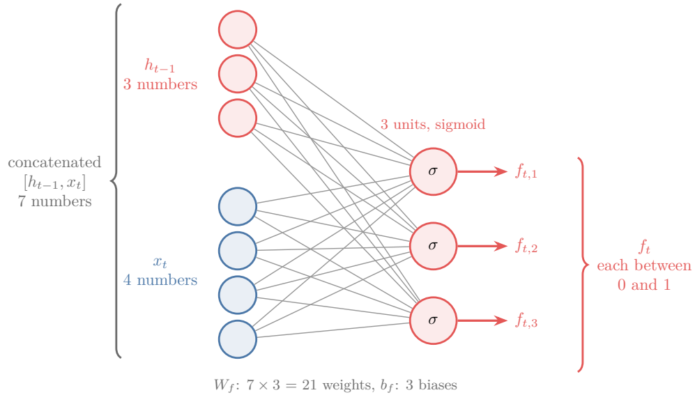
Figure 3: The forget gate's layer. The 3 numbers of h_{t-1} and the 4 numbers of x_t are joined into one input of 7 numbers, fully connected to 3 sigmoid units. Their 3 outputs form f_t
