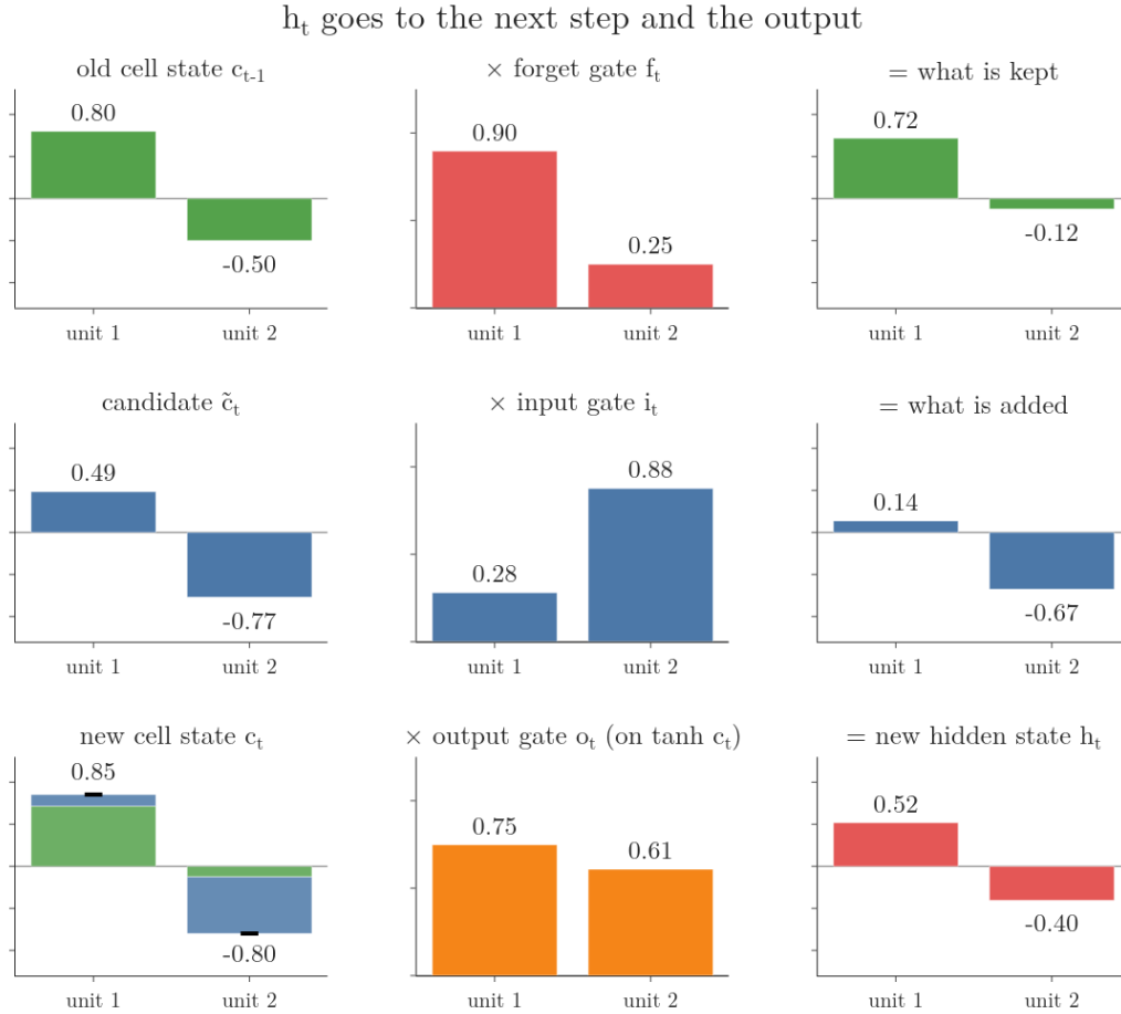
Figure 6: The time step above, one vector per frame. Each row is “value \times gate = result”: the forget gate scales the old cell state, the input gate scales the candidate, and the output gate scales \tanh(c_t) . The new cell state is drawn as what is kept (green) plus what is added (blue)
