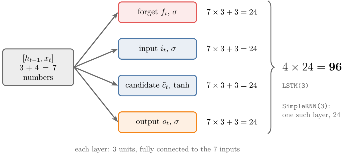
Figure 7: Where the 96 parameters of LSTM(3) on 4 input features come from: four layers, each fully connected from the 7 numbers of [h_{t-1}, x_t] to 3 units, so 7 \times 3 weights plus 3 biases each
