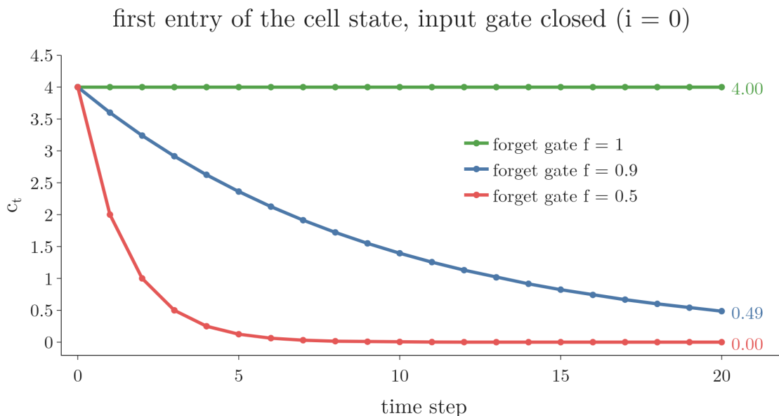
Figure 5: The first entry of the cell state [4, 5, 6] over 20 time steps with the input gate closed, for three forget-gate values. Only f = 1 carries the value unchanged
