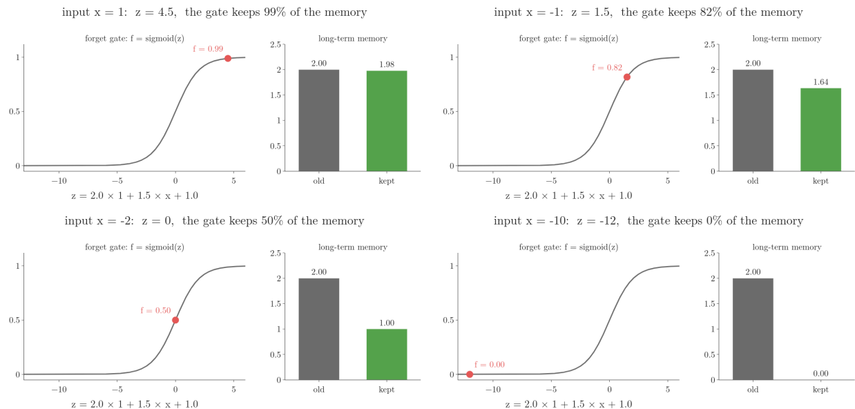
Figure 4: The forget gate of a one-unit LSTM as the input x_t falls from 1 to -10. Left: the gate value f_t on the sigmoid curve. Right: the old long-term memory (grey, 2.00) and what the gate keeps of it (green, f_t \times 2 ). Idea after StatQuest, “Long Short-Term Memory (LSTM), Clearly Explained”, with our own numbers
