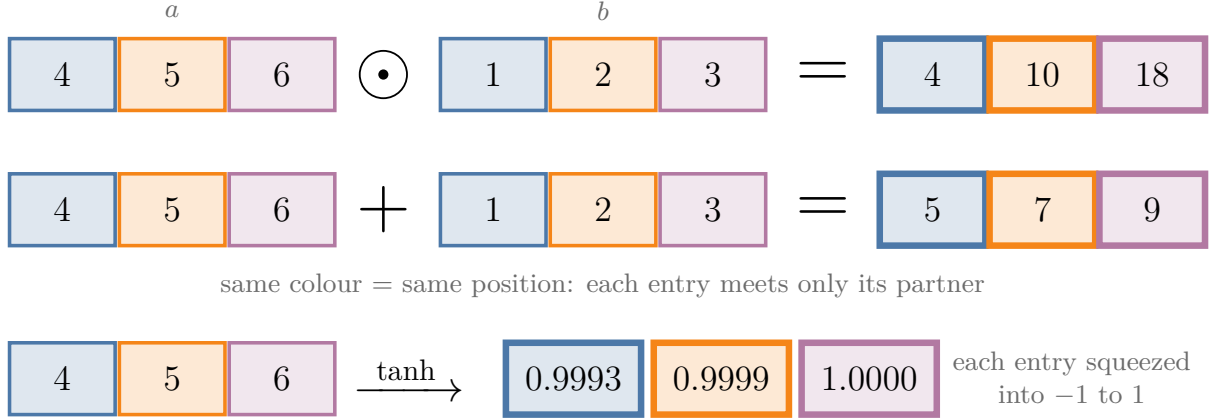
Figure 2: The example above, drawn. Each colour is one position: in a \odot b and a + b , an entry only ever meets the entry of the same colour, and \tanh acts on each entry alone
