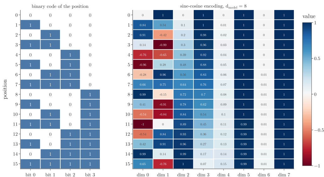
Figure 8: Left: the binary codes of positions 0 to 15; bit 0 flips at every step, bit 3 only once. Right: the sine-cosine encoding of the same positions with d_{\text{model}} = 8 ; dimensions 0 and 1 change fastest, dimensions 6 and 7 barely change
