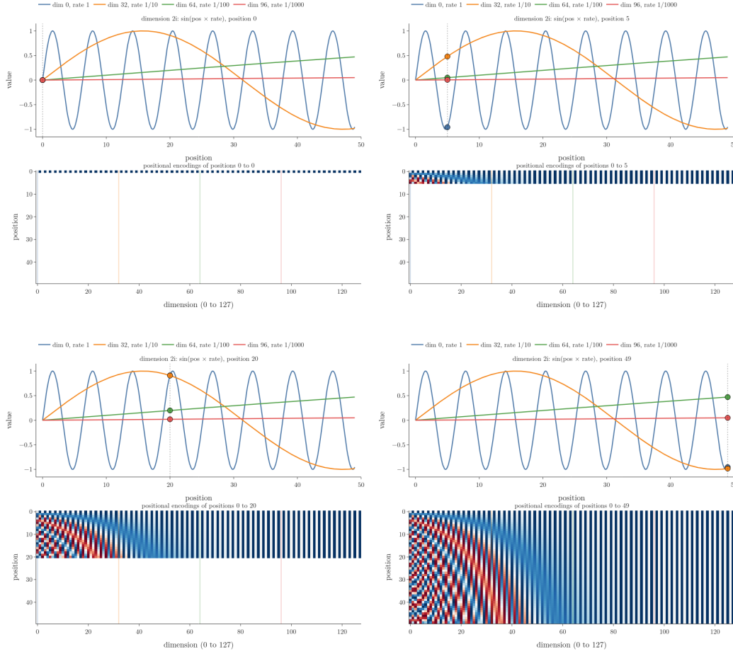
Figure 6: The encoding built one position per frame ( d_{\text{model}} = 128 ). Top: four of the 64 sine waves, with angle rates 1, 1/10, 1/100 and 1/1000; the dots are their values at the current position. Bottom: the rows filled so far; the coloured lines mark the same four dimensions
