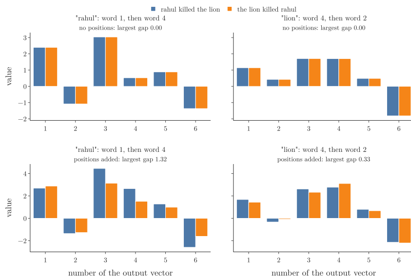
Figure 3: The output vector of “rahul” and of “lion” from the same attention layer, for the two word orders. Top: without positions, the two bars of every pair are equal. Bottom: with positional encodings added to the embeddings, they differ. Idea of swapping the words after StatQuest, “Transformer Neural Networks, ChatGPT’s foundation, Clearly Explained!!!”
