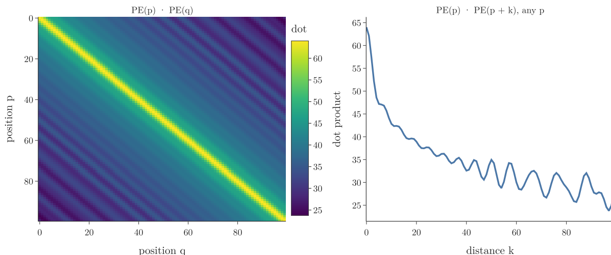
Figure 10: Left: dot products between the encodings of positions 0 to 99; each diagonal, a fixed distance, has one colour. Right: the dot product against the distance k , the same for every starting position
