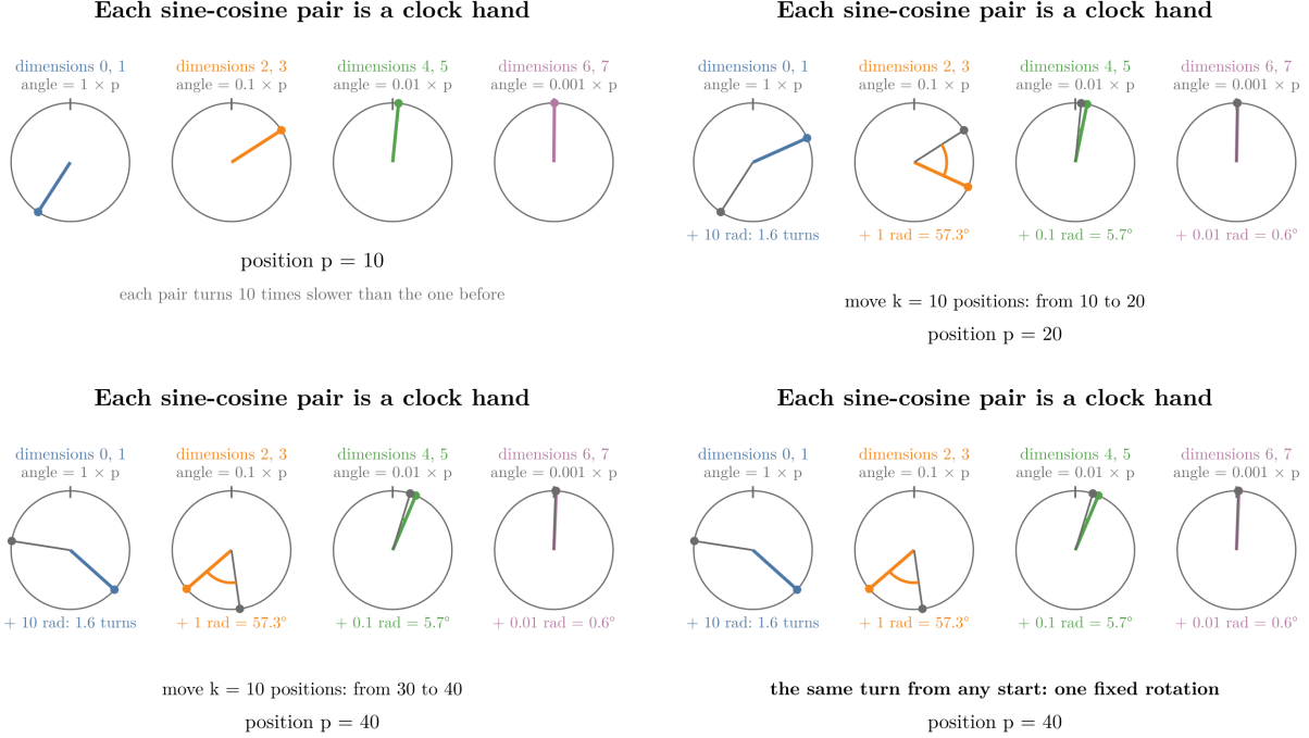
Figure 9: The four sine-cosine pairs of a positional encoding with d_{\text{model}} = 8 as clock hands. Moving 10 positions turns each hand by its own fixed angle (grey: where the hand started), the same from position 10 as from position 30
