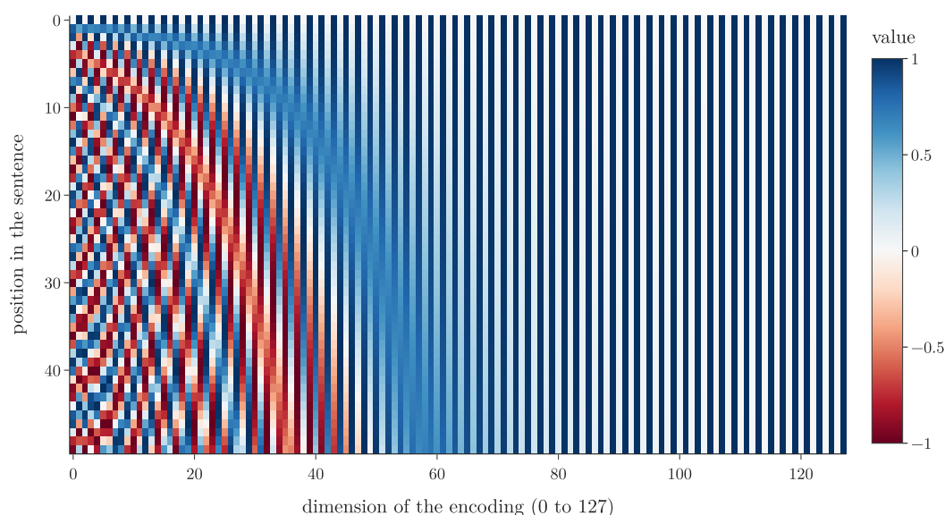
Figure 7: Positional encodings of 50 positions with d_{\text{model}} = 128 . Row 0 alternates 0 and 1; the left dimensions change quickly from row to row, the right ones hardly at all
