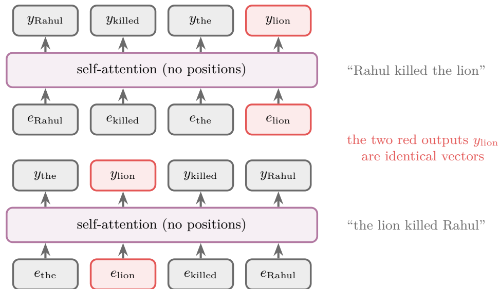
Figure 2: Self-attention with no positions. The two sentences contain the same four embeddings, so the layer returns the same four outputs in a different order; “lion” (red) gets the identical vector in both
