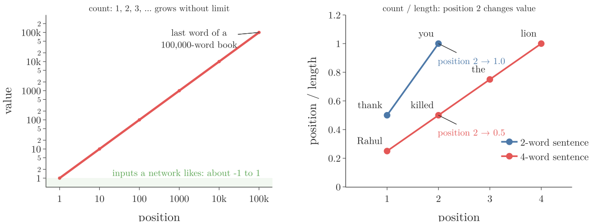
Figure 4: Left: the raw count grows without limit (log scales); the green band is the range a network handles well. Right: dividing by the sentence length keeps the values below 1, but position 2 gets 1.0 in “thank you” and 0.5 in “Rahul killed the lion”
