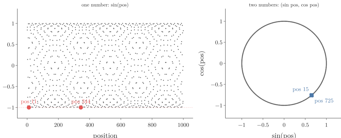
Figure 5: Left: \sin(\text{pos}) for positions 1 to 1,000; positions 11 and 344 (red) sit at almost the same height. Right: with a sine and a cosine, every position is a point on a circle; positions 15 and 725 (blue) still land almost on the same point
