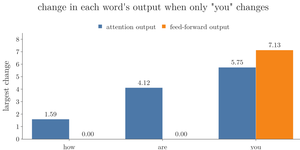
Figure 5: The tiny block of this section, with 5 added to every number of “you”. Blue: how much each word’s attention output changes. Orange: how much each word’s feed-forward output changes
