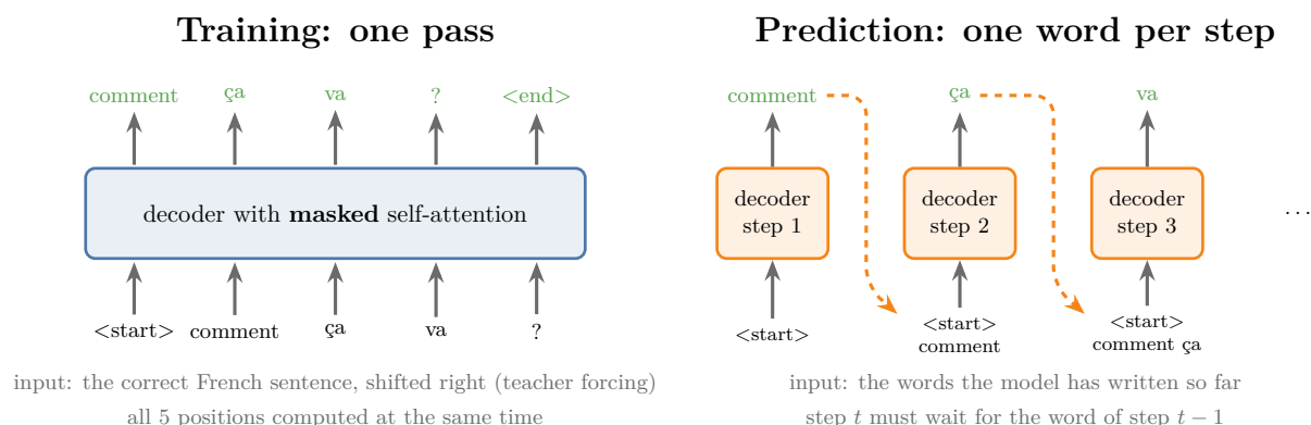
Figure 1: Left: during training the decoder receives the whole correct French sentence, shifted right, and computes every position in one pass. Right: during prediction it writes one word per step, and each step must wait for the word of the step before
