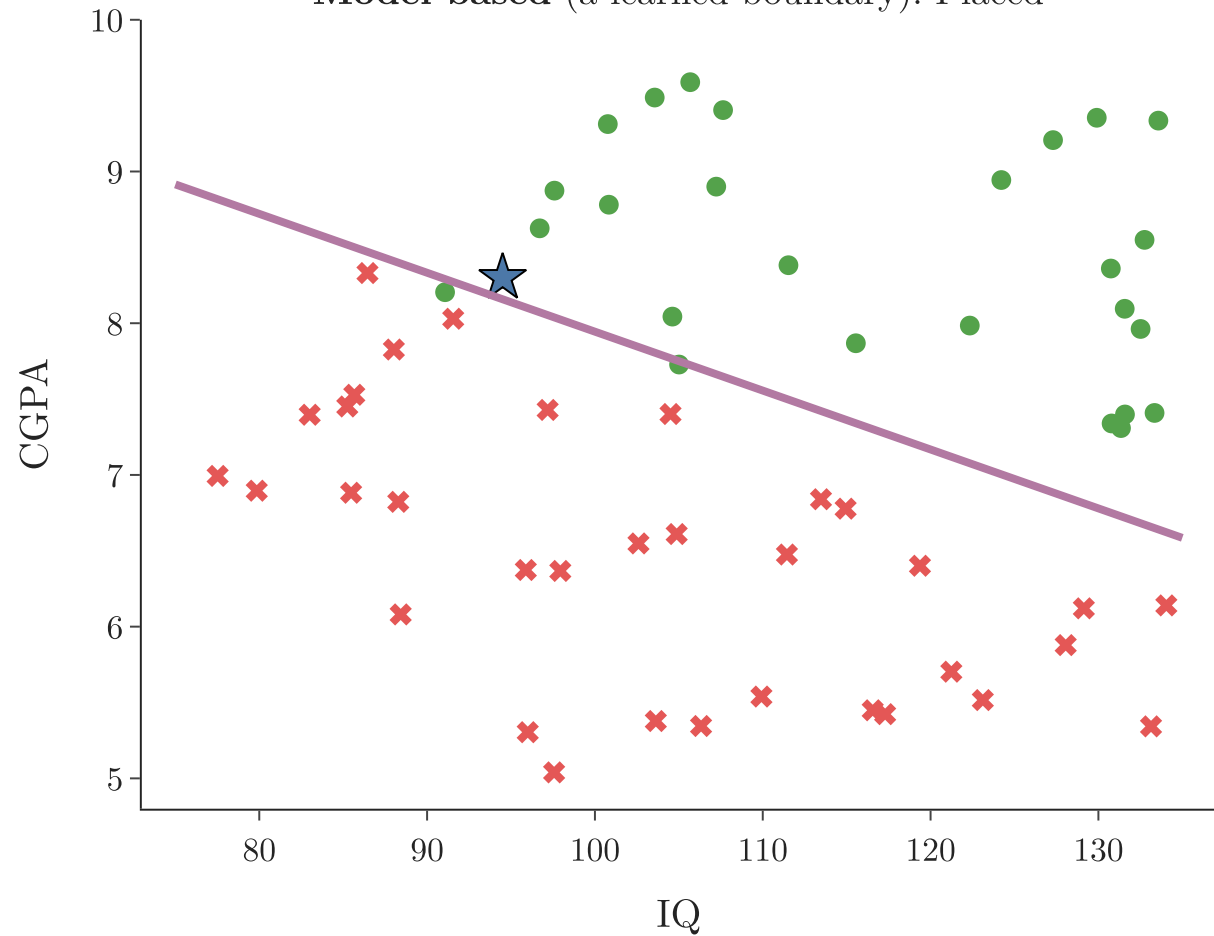
Model-based (a learned boundary): Placed
