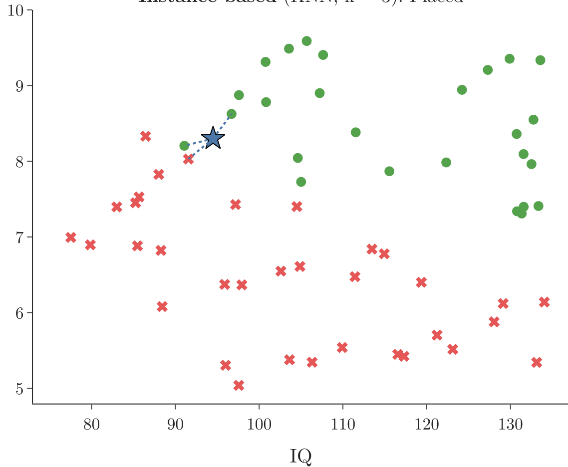
Instance-based (KNN, k = 3 ): Placed
