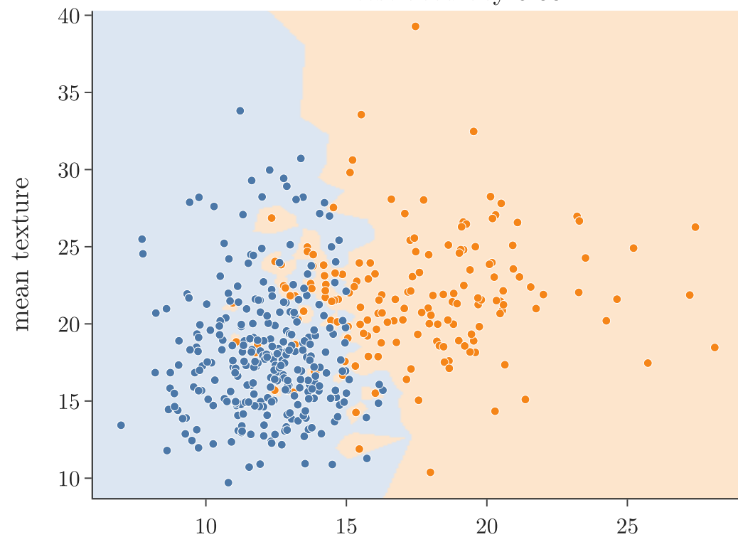
k = 1: test accuracy 0.83
