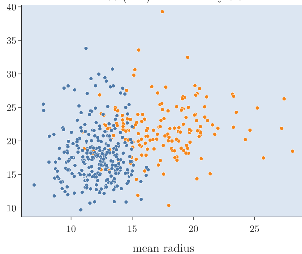
k = 455 (= n): test accuracy 0.61
