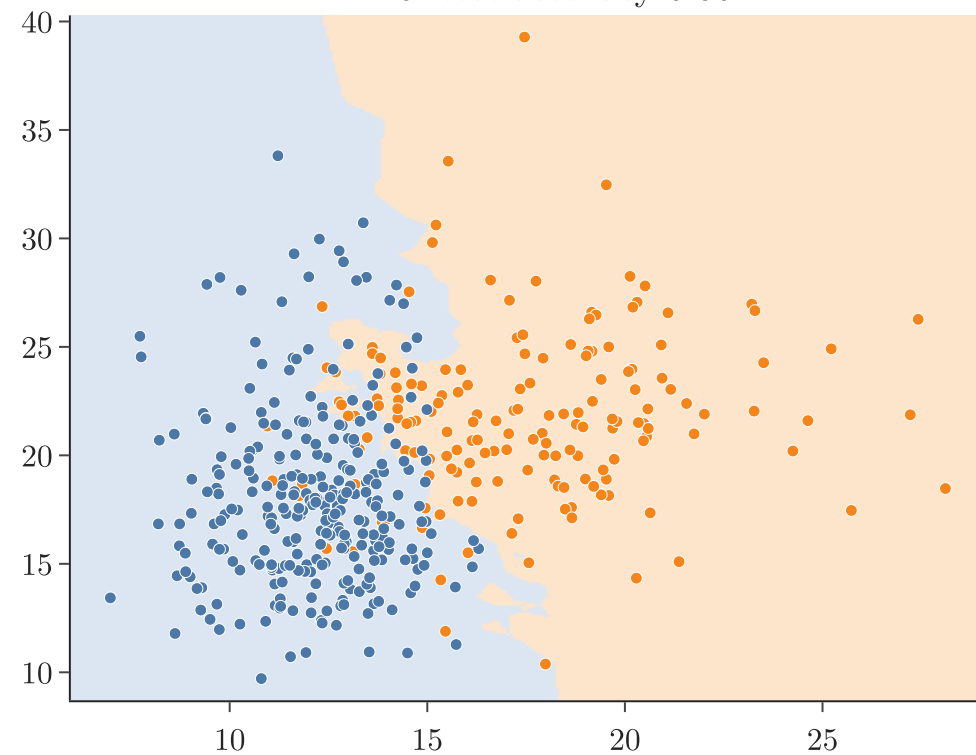
k = 5: test accuracy 0.86
