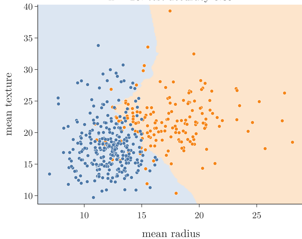
k = 20: test accuracy 0.89
