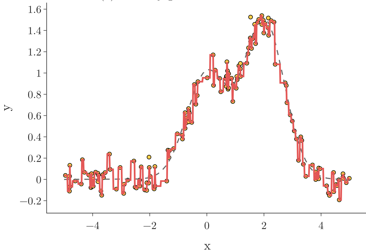
(a) one fully grown tree: test MSE 0.0192
