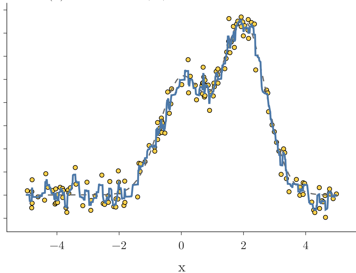
(b) random forest, 1,000 trees: test MSE 0.0140
