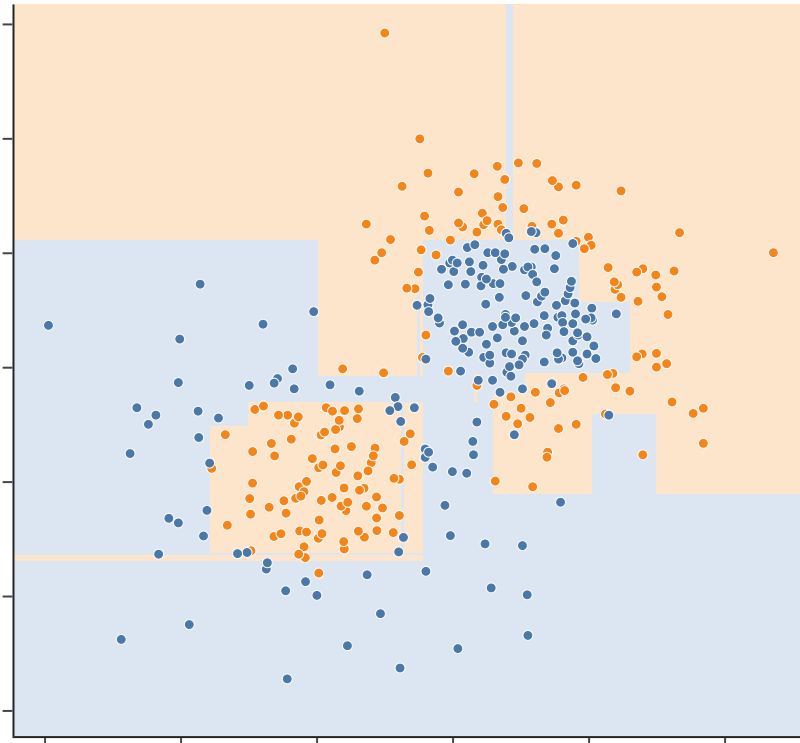
(a) 1 tree: 0.856
