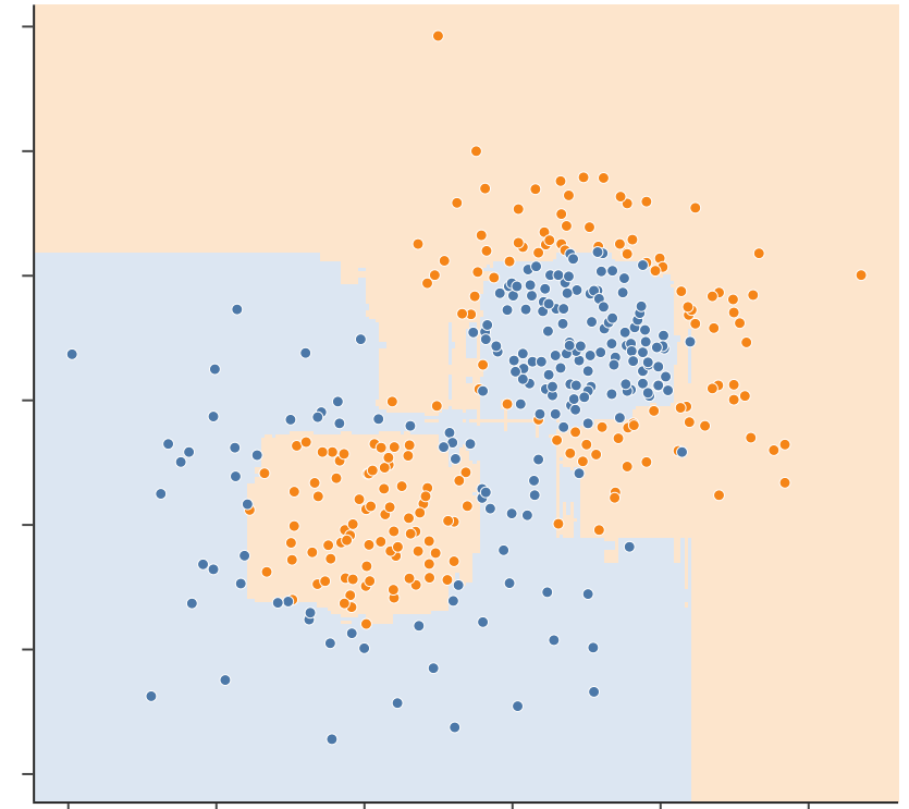
(c) 50 trees: 0.896
