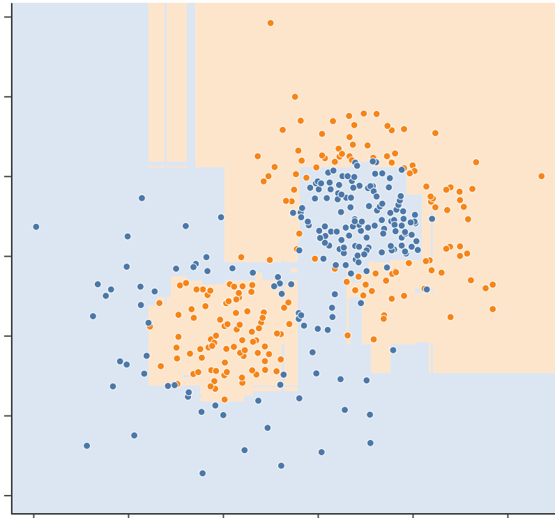
(b) 5 trees: 0.880
