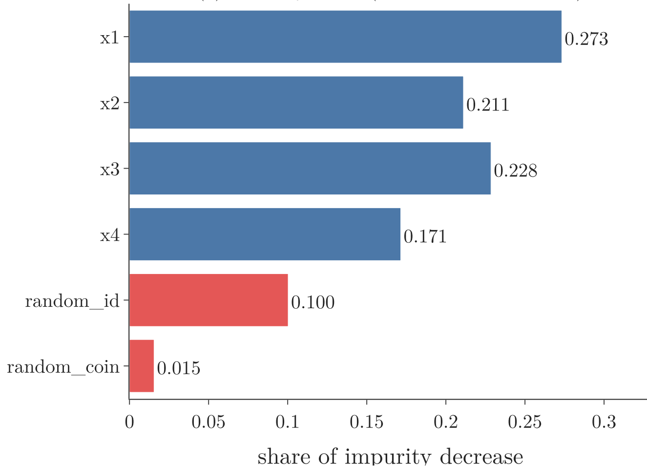
(a) impurity-based (feature_importances_)
