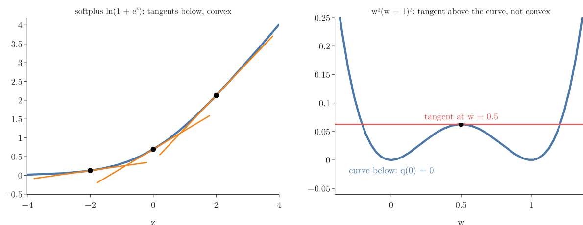
Figure 2: The first-order test. Left: every tangent of softplus lies below the curve, so it is convex. Right: the tangent of w^2(w-1)^2 at w = 0.5 lies above the curve near 0 and 1, so it is not convex
