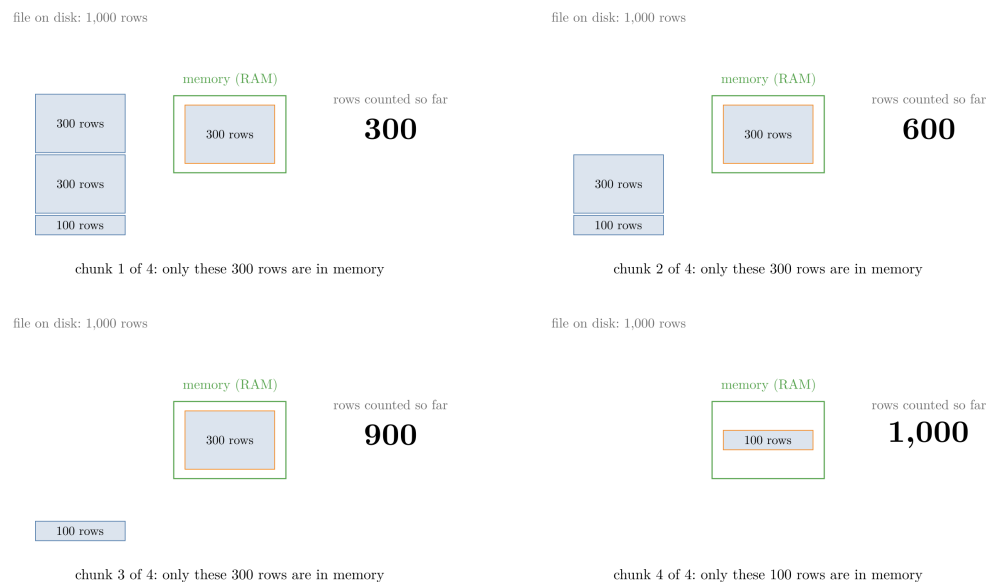
Figure 5: Reading 1,000 rows in chunks of 300
