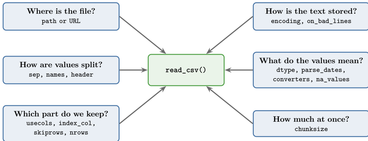
Figure 3: What each read_csv parameter controls
