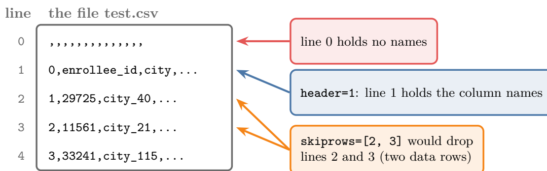
Figure 4: Line numbers in a CSV file, and what header and skiprows refer to
