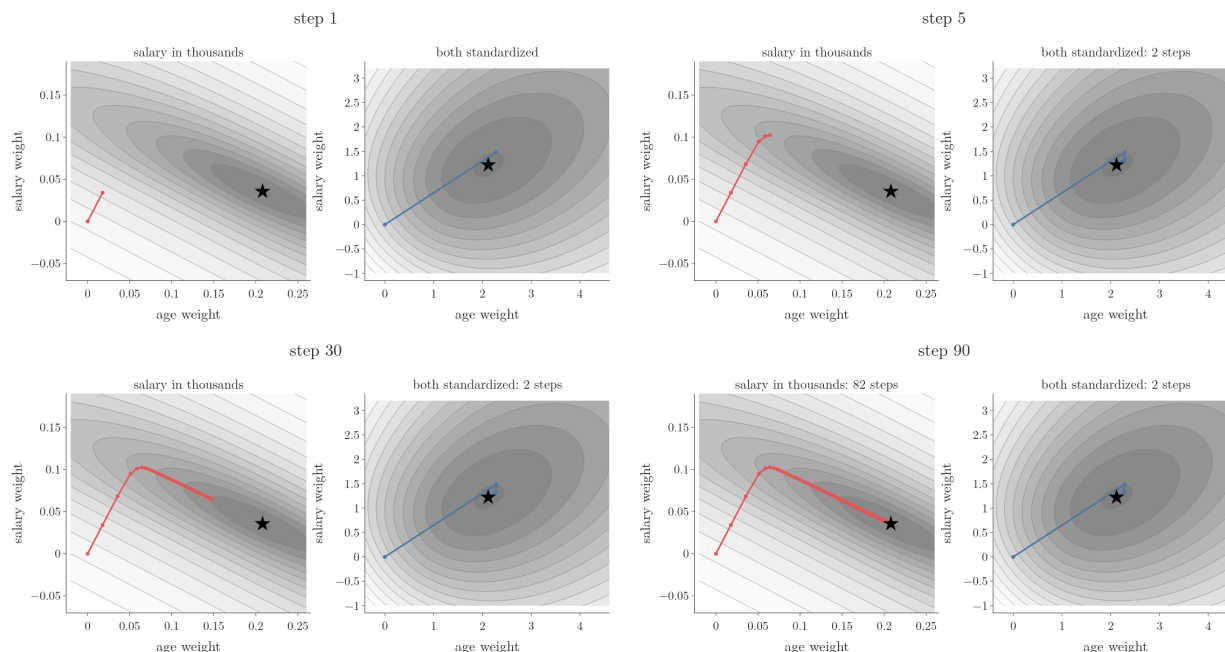
Figure 5: Gradient descent on the loss of one sigmoid node (logistic regression) for our 320 training users, drawn over the age weight and the salary weight, with the bias held at its best value. Both runs start at (0, 0) with a learning rate matched to their surface (1 divided by its steepest curvature at the minimum); the star is the minimum. Left: age in years, salary in thousands. Right: both standardized.
