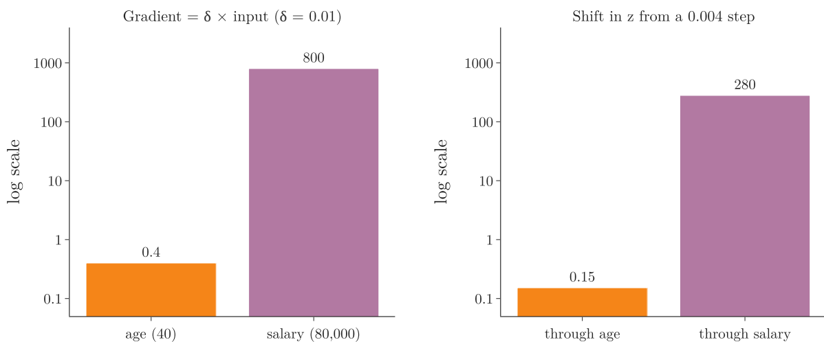
Figure 3: The worked example as bars (log scale). Left: the gradients \delta \cdot x of the age and salary weights for one user. Right: how far one Adam-sized step of 0.004 moves z through a typical age (38) and a typical salary (70,000).
