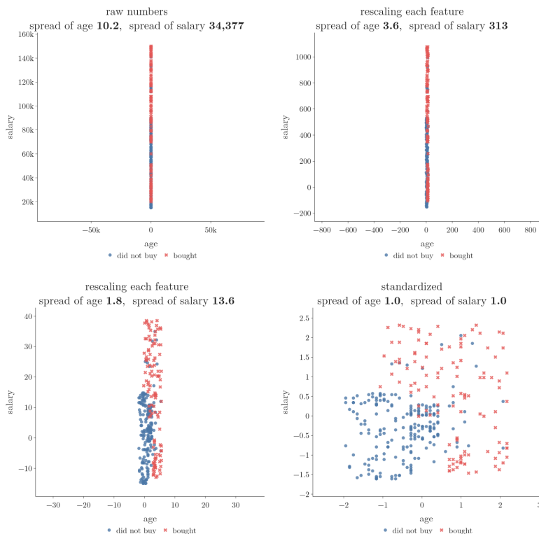
Figure 7: The 320 training users while each feature has its mean removed and is divided by its standard deviation. One unit has the same length on both axes. The title gives the standard deviation (spread) of each feature
