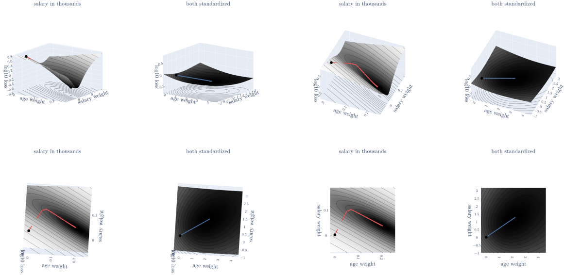
Figure 4: The loss surfaces of the sigmoid node for salary in thousands (left) and both inputs standardized (right), drawn as \log_{10} of the loss. The camera tilts from a side view to the top view; the black lines join points at the same height. Coloured lines: the gradient descent paths of Figure 5; black dot: start (0, 0) ; black diamond: the lowest point
