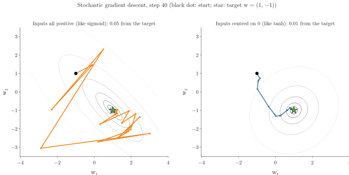
Figure 4: Stochastic gradient descent on one node with two weights. Left: inputs all positive. Right: the same inputs centred on 0. Grey: contours of the loss; black dot: start; star: the target weights.
