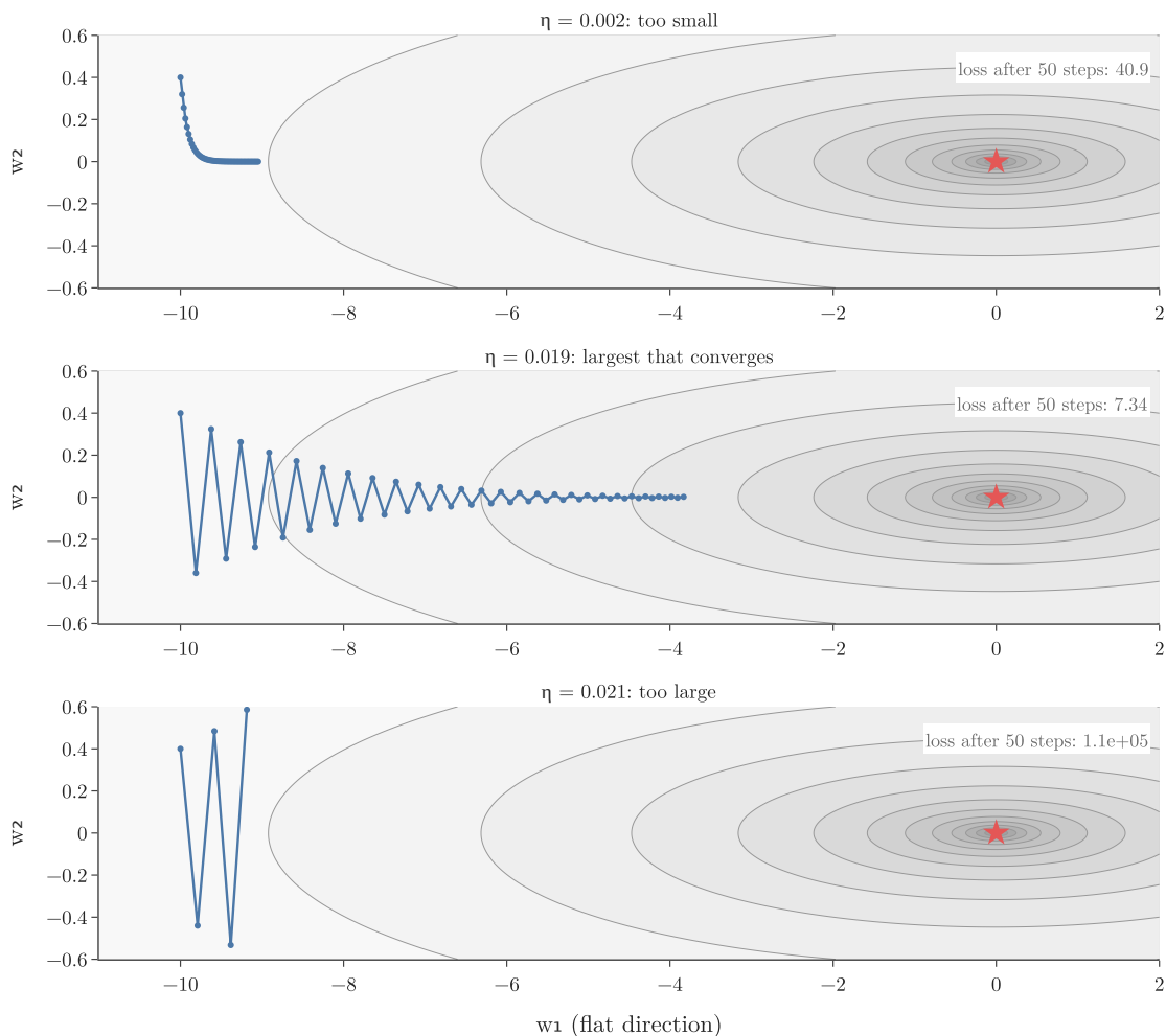
Figure 5: Gradient descent on the valley L = (w_1^2 + 100w_2^2)/2 from (-10, 0.4) , 50 steps each. Top: \eta = 0.002 barely moves along the valley. Middle: \eta = 0.019 zigzags across the valley and is still far from the minimum (star). Bottom: \eta = 0.021 bounces out of the valley
