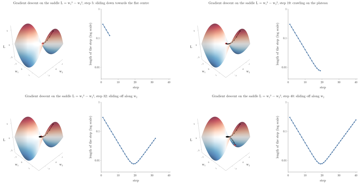
Figure 6: Gradient descent near a saddle point. Left: the surface L = w_1^2 - w_2^2 with the path (red dot: current position). Right: the length of each step, on a log scale
