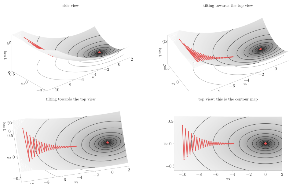
Figure 4: The valley as a surface, seen from the side and then tilted to the top view. Red: gradient descent with \eta = 0.019 from (-10, 0.4) , 50 steps. Height is the loss L . Thin lines join points of equal height, on the surface and dropped to the floor; each line is about double the one inside it. The walls go higher than drawn
