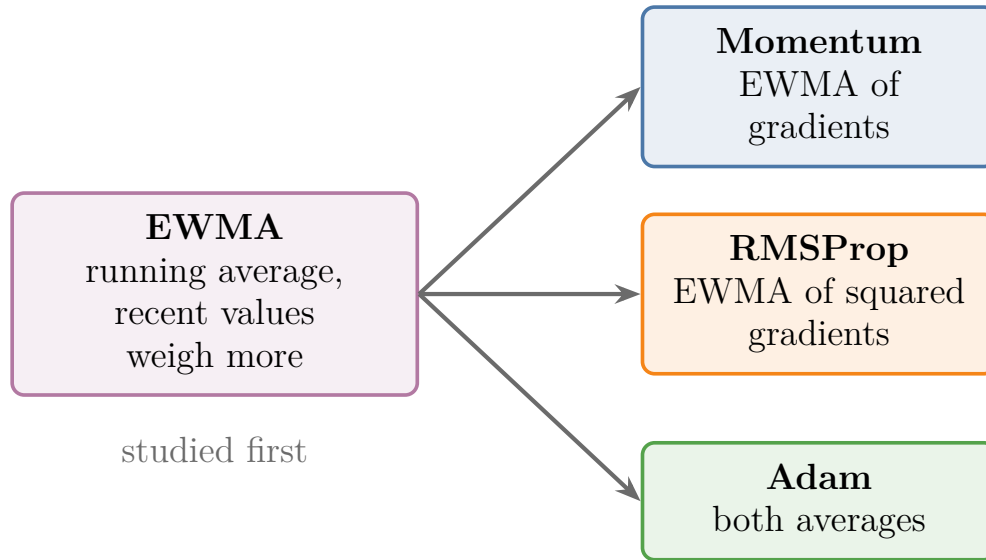
Figure 7: The EWMA is the shared tool: Momentum averages the gradients, RMSProp the squared gradients, and Adam keeps both averages
