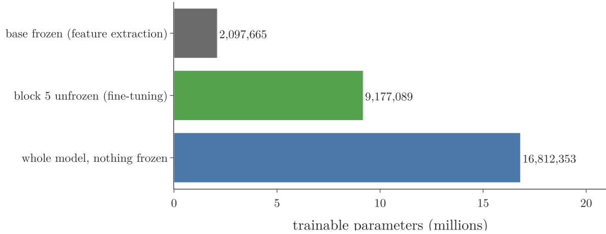
Figure 6: Trainable parameters of the same model under the three settings of trainable (Notebook).
