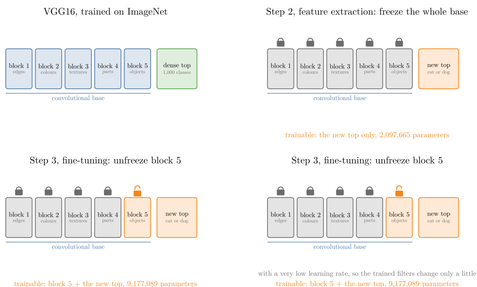
Figure 4: Transfer learning on VGG16 in three steps. The ImageNet top is cut off and a new top is added; every block of the convolutional base is frozen (feature extraction, 2,097,665 trainable parameters); then block 5 is unfrozen (fine-tuning, 9,177,089 trainable parameters)
