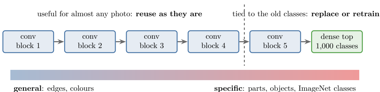
Figure 3: VGG16’s layers from general to specific. The early blocks find edges and colours, useful for any photo; the last block and the dense top hold the features tied to ImageNet’s classes.
