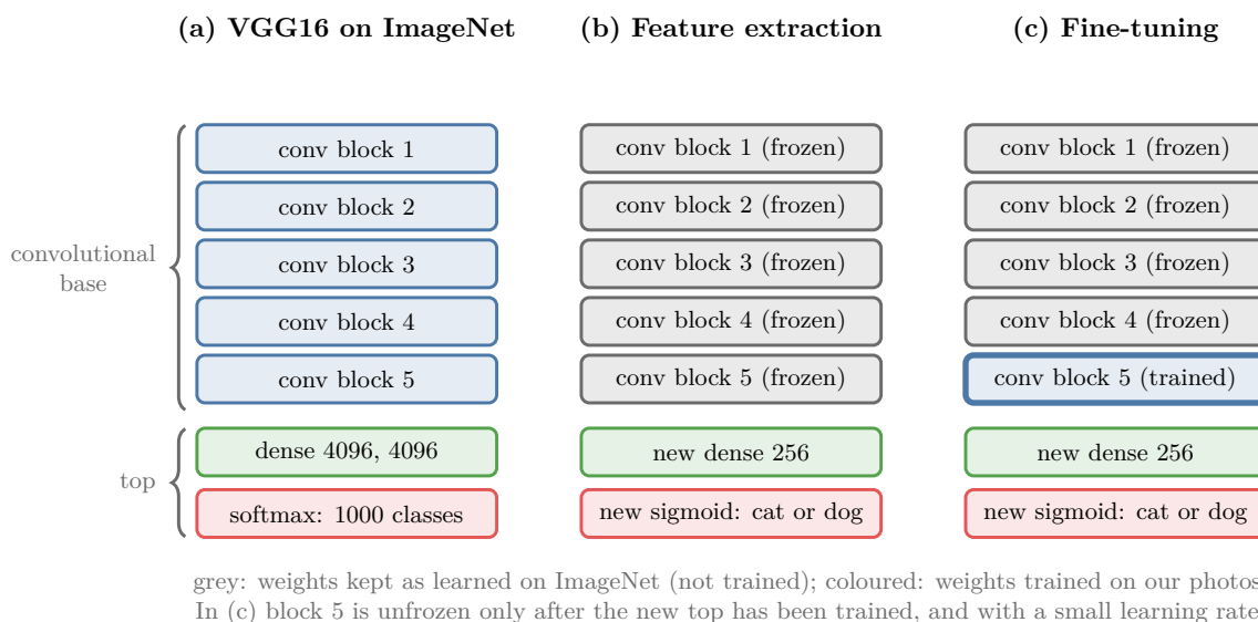
Figure 2: (a) VGG16 as trained on ImageNet. (b) Feature extraction: the whole convolutional base is frozen, and only a new top is trained. (c) Fine-tuning: the last convolution block is also trained, after the new top
