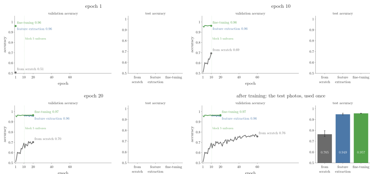
Figure 7: Validation accuracy drawn epoch by epoch (left; mean of 3 seeds), then the test accuracy (right; bars: mean, whiskers: lowest and highest of 3 seeds). The dotted line marks where fine-tuning unfreezes block 5
