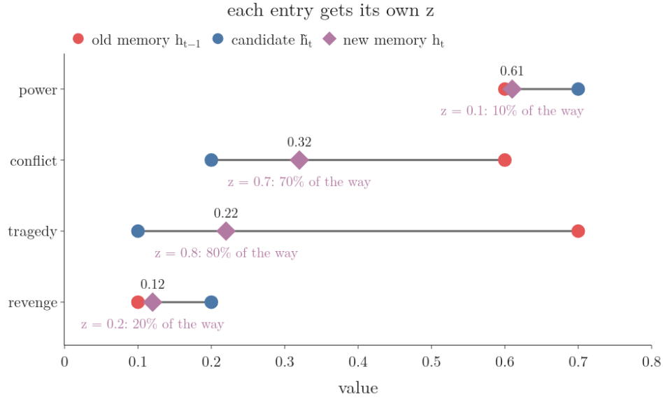
Figure 5: Sentence 4 of the story. For each aspect, the segment runs from the old memory (red) to the candidate (blue), and the new memory (diamond) slides along it. With z = 0 the diamond stays on the old memory; with z = 1 it lands on the candidate; at the end each aspect gets its own z , the update-gate values of section 8.3
