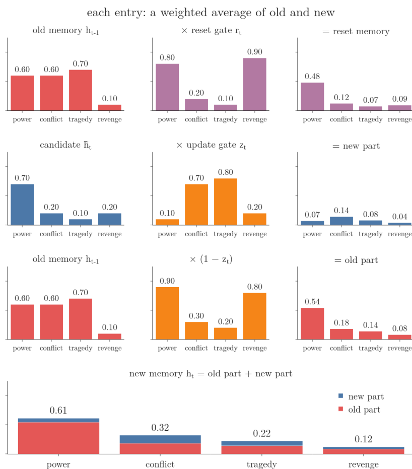
Figure 7: The four steps for sentence 4 of the story, one vector per frame. Row 1: the reset gate scales the old memory. Row 2: the update gate scales the candidate. Row 3: 1 - z_t scales the old memory. Bottom: the new memory, old part (red) plus new part (blue)
