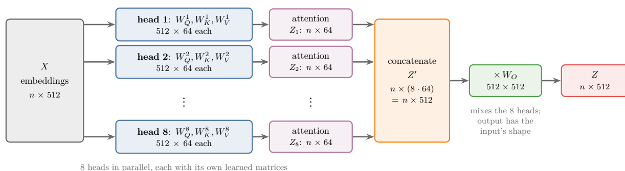
Figure 1: Multi-head attention in the transformer: 8 heads, each with its own W_Q^i, W_K^i, W_V^i , work in parallel on the same embeddings. Their outputs are concatenated and multiplied by W_O , which gives back one 512-number vector per word
