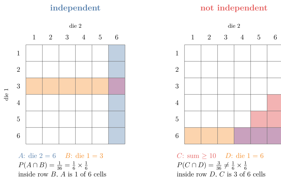
Figure 2: The 36 outcomes of two dice. Purple cells are in both events. Left: row B and column A cross in one cell, so P(A \cap B) = 1/36 = P(A) \times P(B) . Right: the “sum at least 10” cells crowd into row D , so the product rule fails
