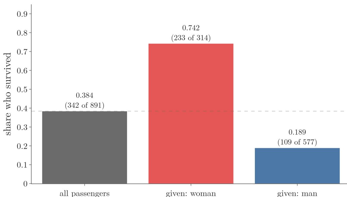
Figure 5: Survival on the Titanic: the share who survived among all 891 passengers (0.384, dashed line), among the 314 women (0.742) and among the 577 men (0.189).
