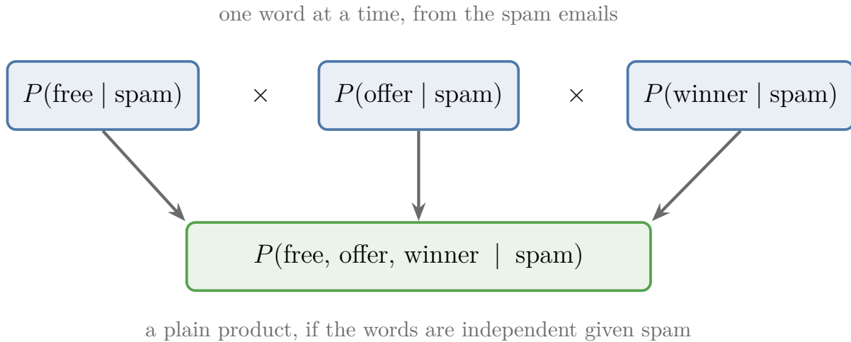
Figure 6: Under independence, the probability of all three words given spam is the product of the three single-word probabilities
