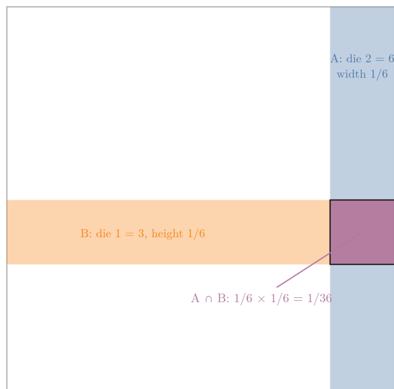
Figure 1: The product rule as areas. The square is the sample space (area 1); A is a band of width 1/6 , B a band of height 1/6 , and their overlap is a 1/6 \times 1/6 rectangle: P(A \cap B) = 1/36 .
