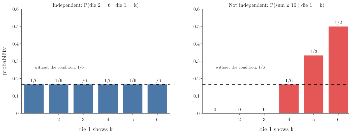
Figure 4: Conditioning on die 1 leaves one event unchanged and changes the other
