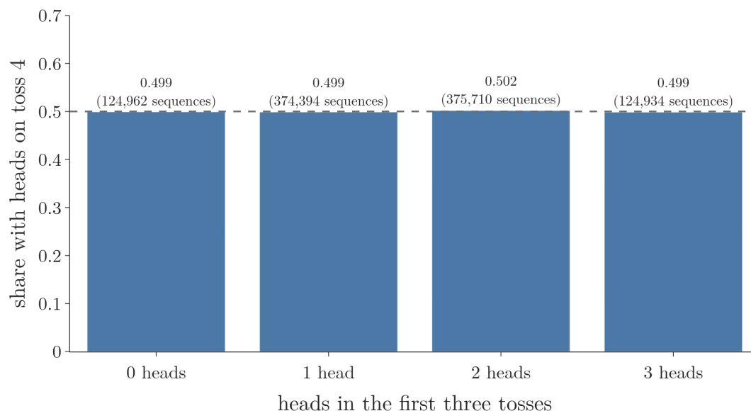
Figure 3: One million sequences of four fair coin tosses. For each number of heads among the first three tosses, the share of sequences with heads on the fourth toss: 0.499, 0.499, 0.502 and 0.499.
