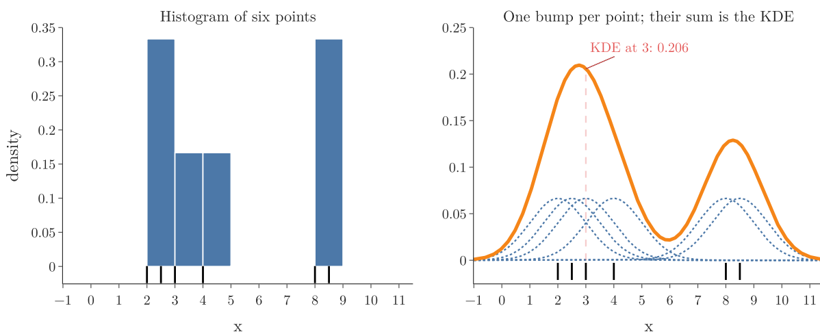
Figure 5: KDE by hand: a Gaussian bump of bandwidth 1 on each of six points, already divided by 6 (dotted); their sum is the KDE (orange)
