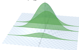
Figure 5: The bell lifted to a round bell-shaped surface: its volume by thin cylindrical shells is pi, by slices it is C^2 , so C = square root of pi (idea after 3Blue1Brown, “Why \pi is in the normal distribution (beyond integral tricks)”)
