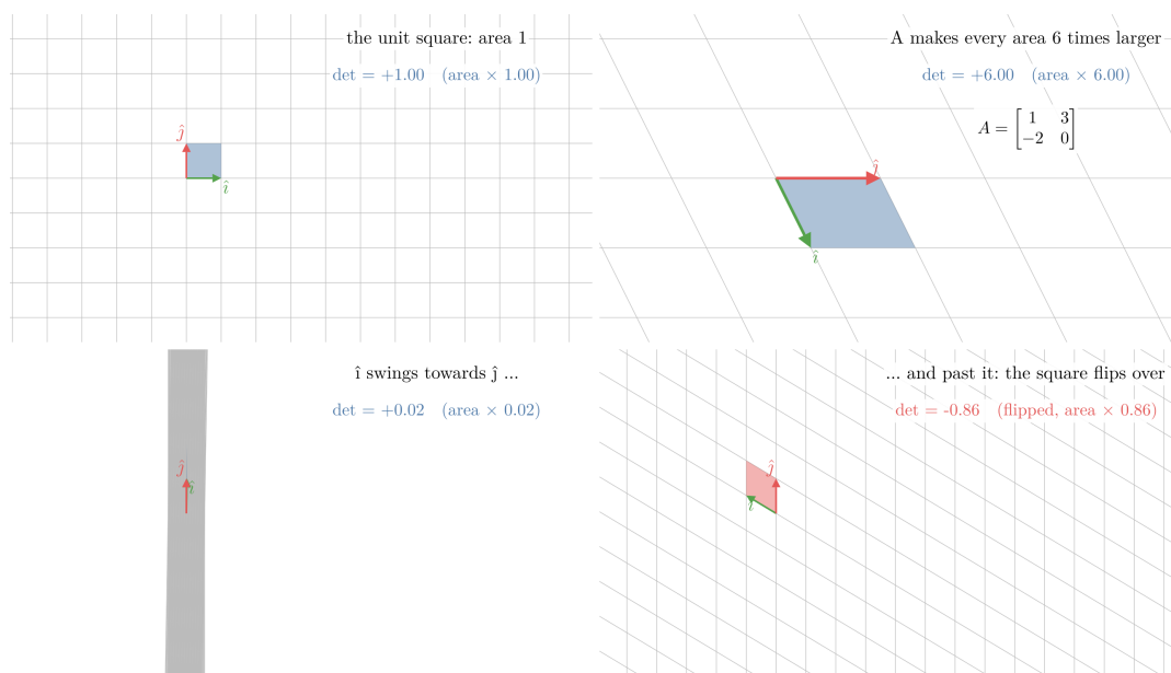
Figure 6: The unit square under A (rows [1, 3] , [-2, 0] ) becomes a parallelogram of area 6. Then, back on the unit square, \hat{i} swings towards \hat{j} : the area shrinks to 0 when they line up, and past that point the square flips over and the determinant turns negative (red). Idea after 3Blue1Brown, “The determinant | Chapter 6, Essence of linear algebra”
