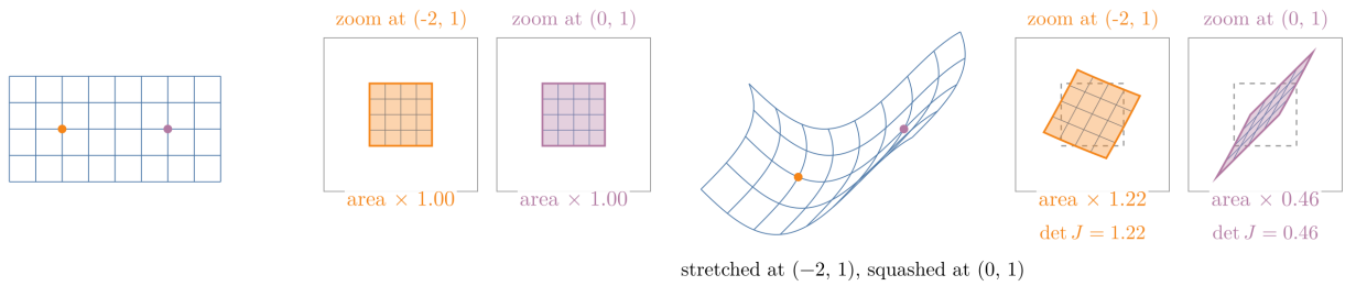
Figure 8: The map \mathbf{g}(x, y) = (x + \sin y, y + \sin x) bends a grid. Each inset follows a tiny square (dashed) while the map plays: at (-2, 1) its image grows to 1.22 times its area, at (0, 1) it shrinks to 0.46 times. Idea after Khan Academy, “The Jacobian Determinant”
