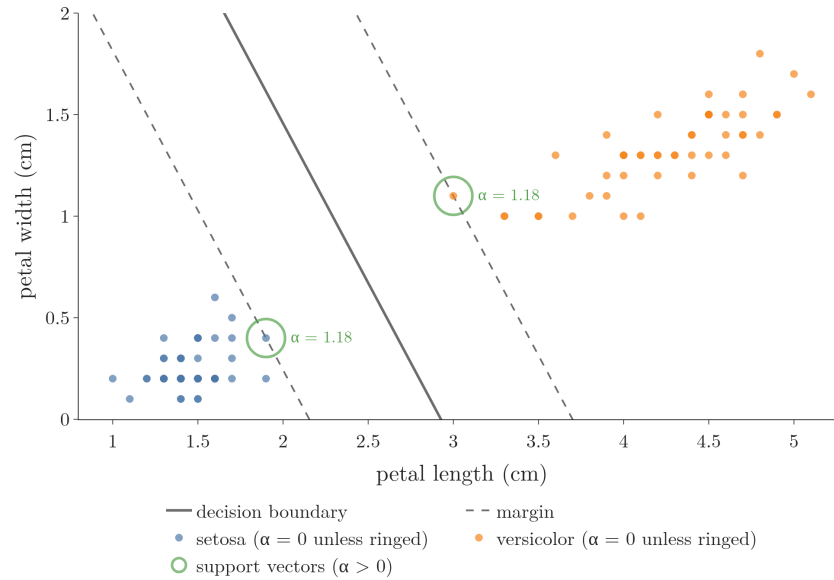
Figure 11: The hard-margin linear SVM on 100 Iris flowers (petal length and width). Rings: the support vectors, the only flowers with a nonzero dual multiplier ( \alpha = 1.18 each). Every other flower has \alpha = 0 .
