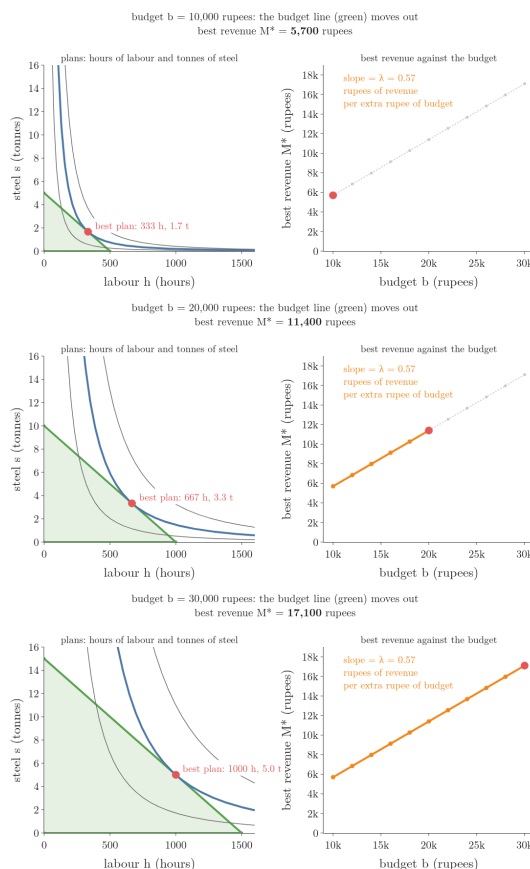
Figure 7: Left: plans of labour and steel. The budget line (green) moves out as the budget grows; the best plan (red) is where a revenue contour (blue) touches it. Right: the best revenue against the budget, a line of slope \lambda = 0.57 . Numbers after Khan Academy, “Lagrange multiplier example, part 1” and “Meaning of Lagrange multiplier”
