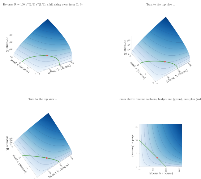
Figure 6: The factory's revenue R = 100 h^{2/3} s^{1/3} as a surface over labour h and steel s , with the budget line 20h + 2000s = 20,000 lifted onto it (green) and the best plan (red, R = 11,400 ). Last frame: the same surface from above, as revenue contours
