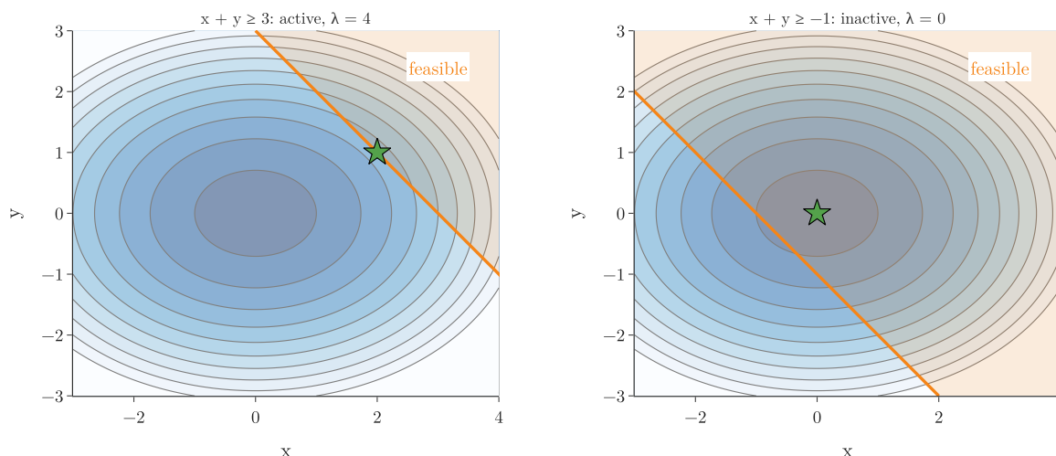
Figure 8: Minimising x^2 + 2y^2 with one inequality constraint; the feasible region is shaded and the star is the answer. Left: x + y \geq 3 cuts off the unconstrained minimum, so the answer lies on the boundary (active, \lambda = 4 ). Right: x + y \geq -1 already contains the unconstrained minimum (inactive, \lambda = 0 )
