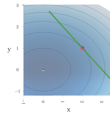
Figure 1: The bowl f = x^2 + 2y^2 with the line x + y = 3 lifted onto it (green). The answer is the lowest point of the green curve, above (2, 1) at height 6. Last frames: the same picture from above, as contour rings and a line. Idea after Khan Academy, “Constrained optimization introduction”; our own problem
