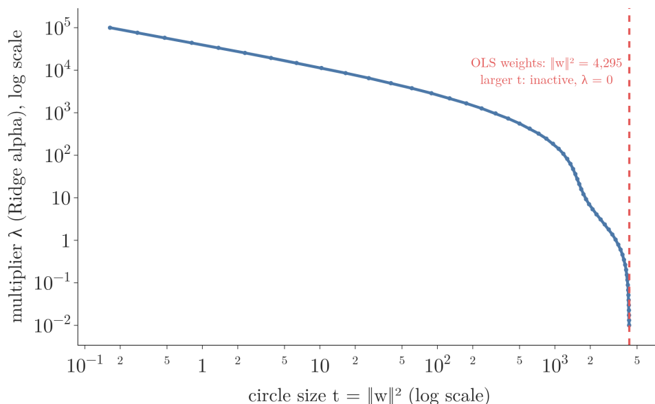
Figure 10: Ridge on the diabetes data (10 standardised features, 442 patients). Each point is one penalty strength \lambda and the size t of the Ridge weights it produces. Small circles need large multipliers; \lambda falls towards 0 as t nears the size of the OLS weights (dashed).
