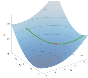
Figure 1: The bowl f = x^2 + 2y^2 with the line x + y = 3 lifted onto it (green). The answer is the lowest point of the green curve, above (2, 1) at height 6. Last frames: the same picture from above, as contour rings and a line. Idea after Khan Academy, “Constrained optimization introduction”; our own problem
