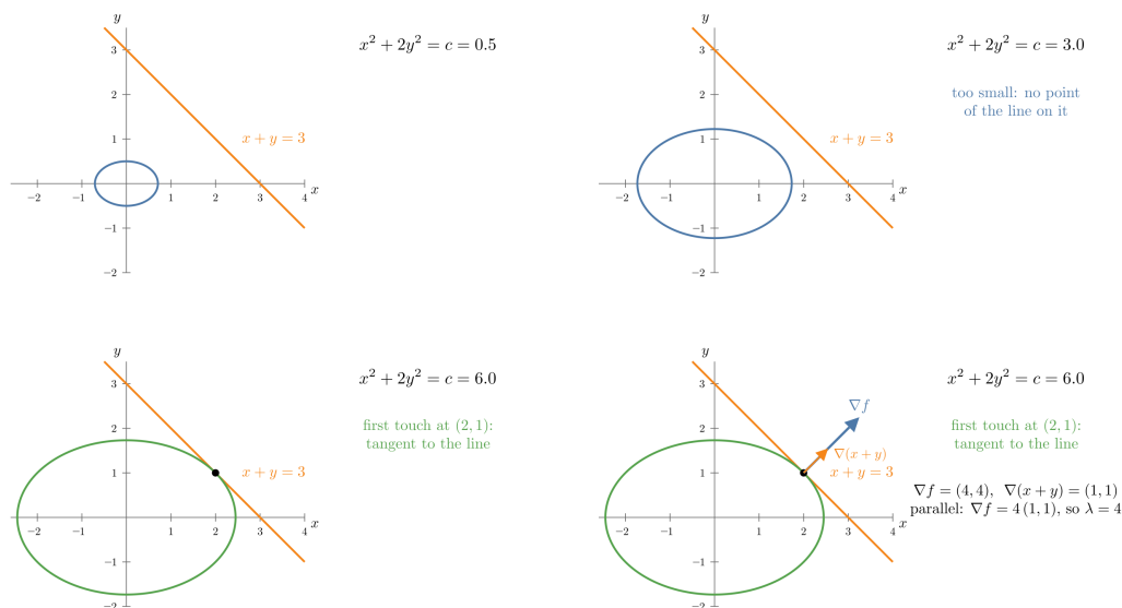
Figure 2: Minimising f = x^2 + 2y^2 on the line x + y = 3 : the level curve f = c grows until it first touches the line at (2, 1) , where the two gradients are parallel. Key frames: c = 0.5 , c = 3 , the first touch at c = 6 , and the gradients
