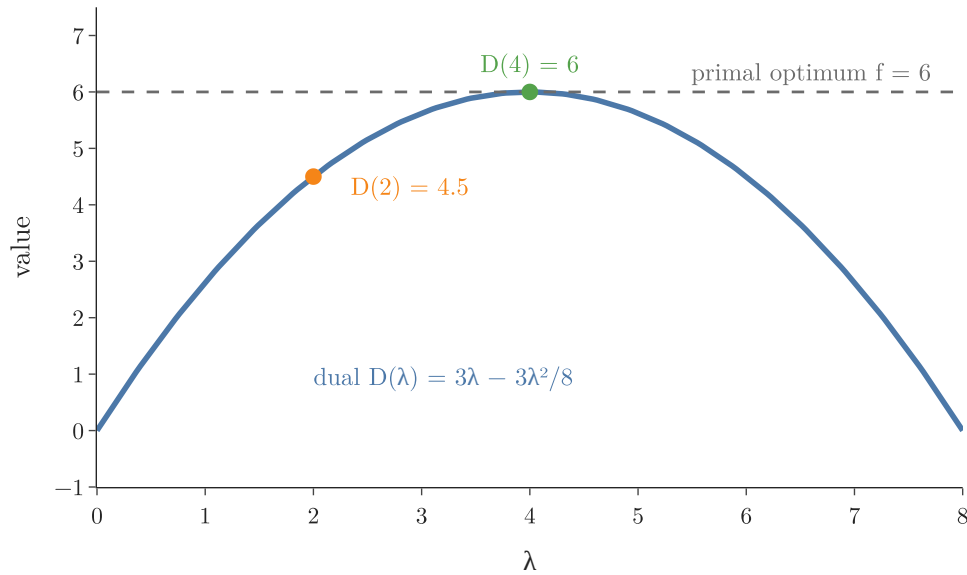
Figure 9: The dual function D(\lambda) = 3\lambda - 3\lambda^2/8 (blue) stays below the primal optimum 6 (dashed) for every \lambda and touches it at \lambda = 4
