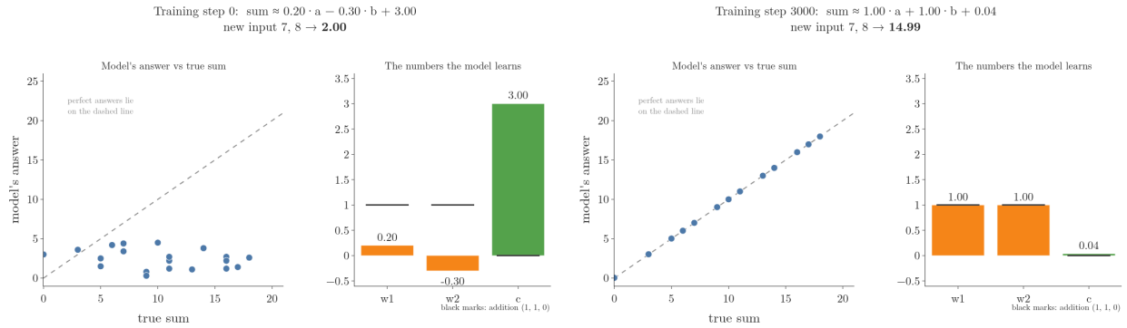
Figure 4: Training a model on 20 pairs of numbers and their sums. Left: each dot is one pair, the model’s answer against the true sum. Right: the three parameters, with black marks at 1, 1 and 0.
