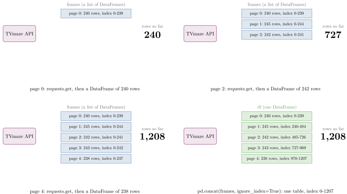
Figure 6: Five pages fetched one by one, then joined into one table
