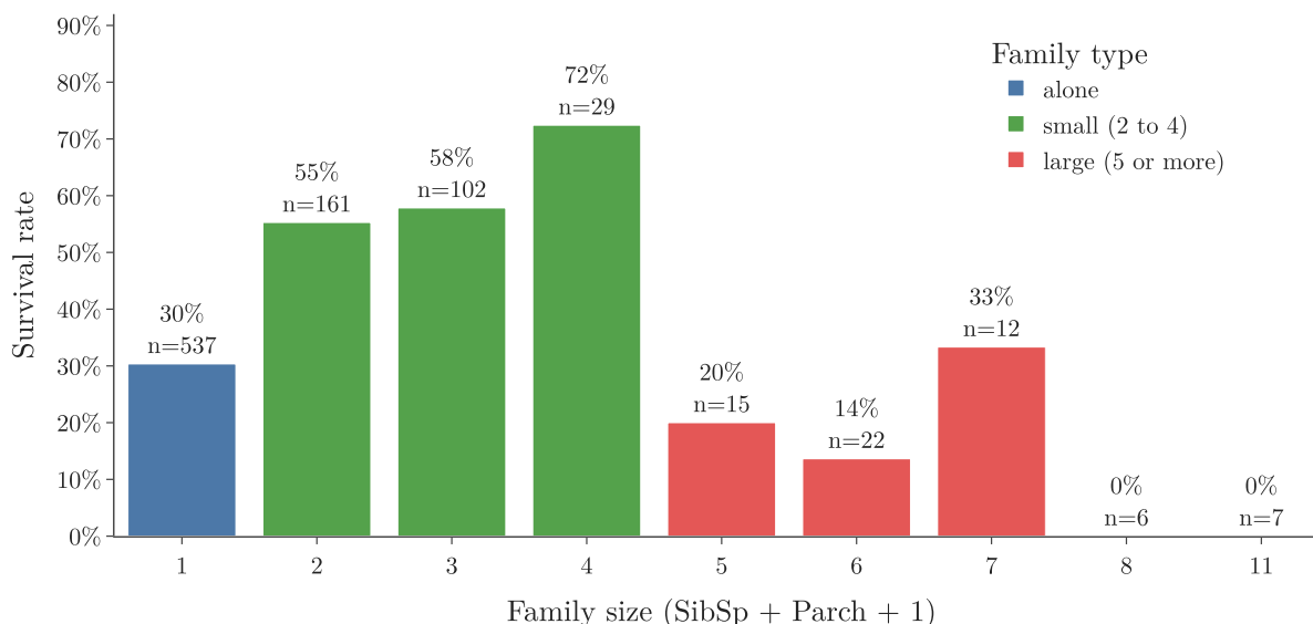
Figure 3: Survival rate for each family size, coloured by family type (all 891 passengers)
