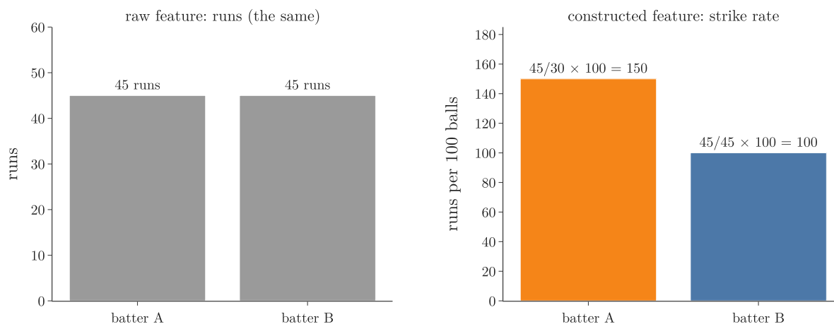
Figure 4: Illustrative numbers: two batters with 45 runs each. The raw runs are equal; the constructed strike rate is 150 for 30 balls and 100 for 45 balls.
