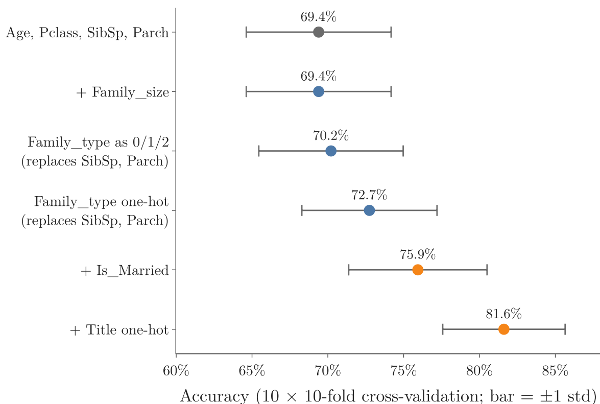
Figure 8: Cross-validated accuracy for each set of features. Dot colour: grey for the baseline, blue for construction, orange for splitting. The grey whiskers show \pm 1 standard deviation of the 100 single-fold scores
