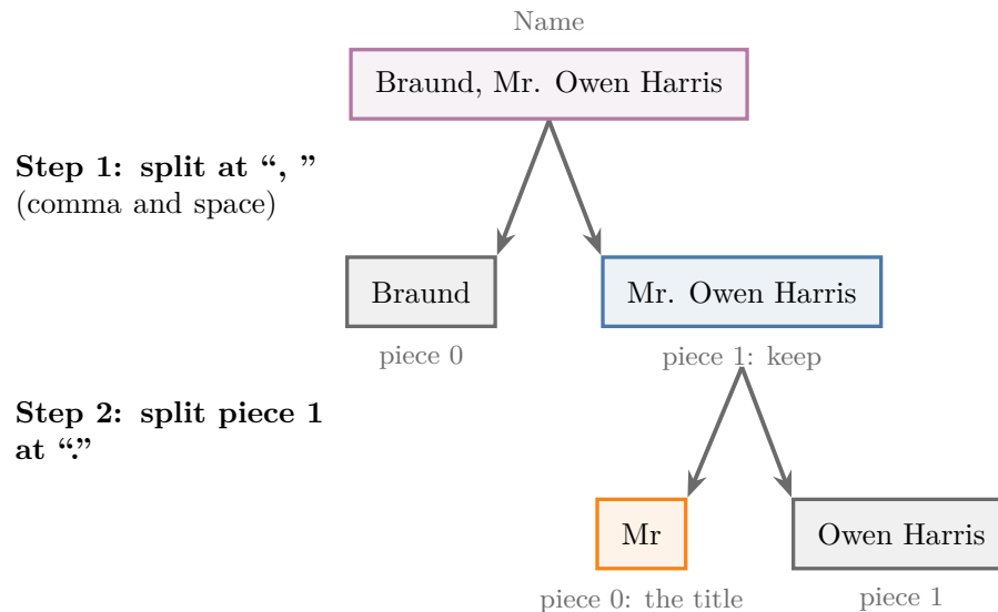
Figure 6: Two splits pull the title out of a name
