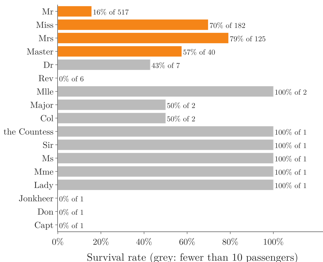
Figure 7: Survival rate for each title; titles with fewer than 10 passengers in grey
