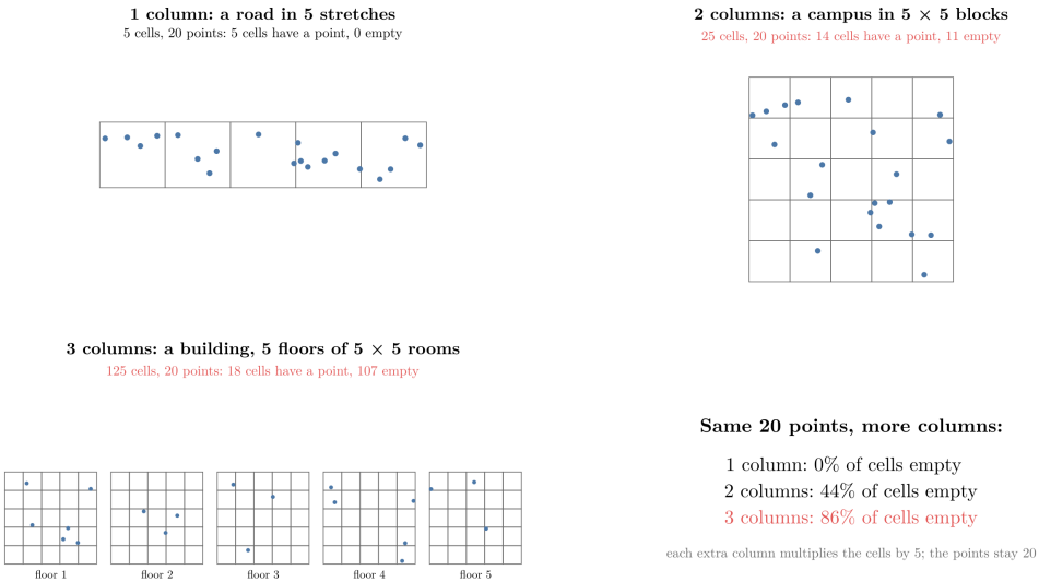
Figure 3: The same 20 points in 1, 2 and 3 features
