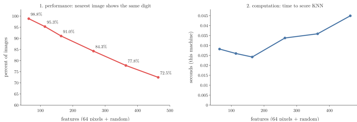
Figure 5: The digits data with useless random features added. Left: the share of images whose nearest other image shows the same digit. Right: the time to score KNN with 5-fold cross-validation (best of 3 runs; machine dependent).
