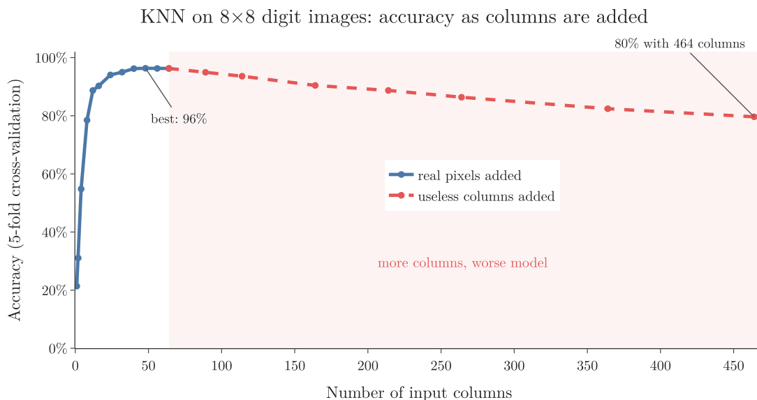
Figure 2: KNN accuracy as features are added (real measurement)
