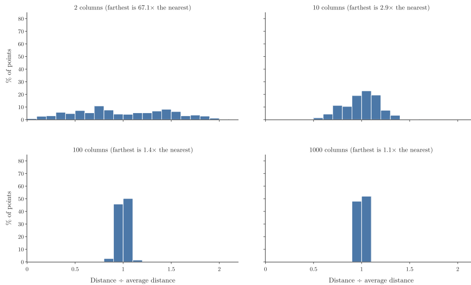
Figure 4: Distances from one point to 500 others, in 2 to 1,000 features
