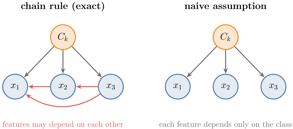
Figure 4: Who depends on whom, for three features. Left: the chain rule allows every feature to depend on the class and on the other features (red arrows). Right: the naive assumption keeps only the arrows from the class
