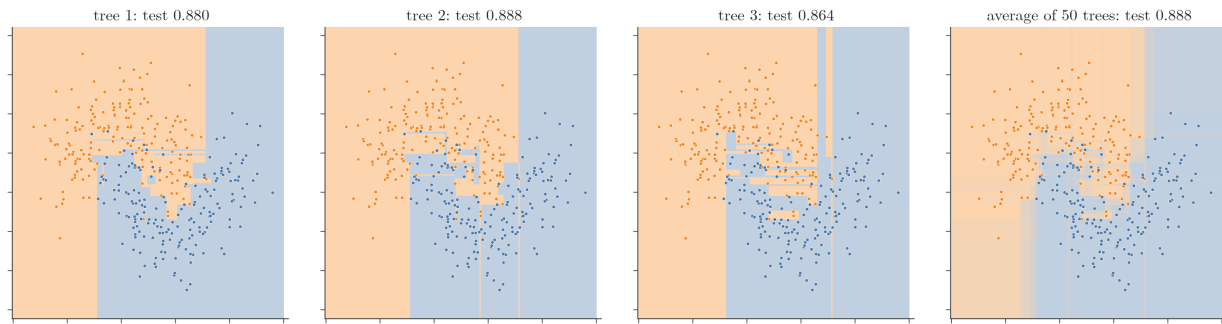
Figure 6: Fully grown trees with max_features = 1 on the moons training data. Three trees with different random seeds draw different surfaces (test accuracy 0.880, 0.888, 0.864); the average vote of 50 such trees (right) scores 0.888.
