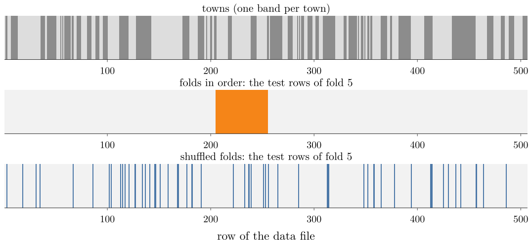
Figure 5: The 506 Boston rows in file order. Top: the towns, one band each. Middle: the test rows of one of 10 folds cut in order, a block of whole towns. Bottom: the test rows of one of 10 shuffled folds, spread across all towns
