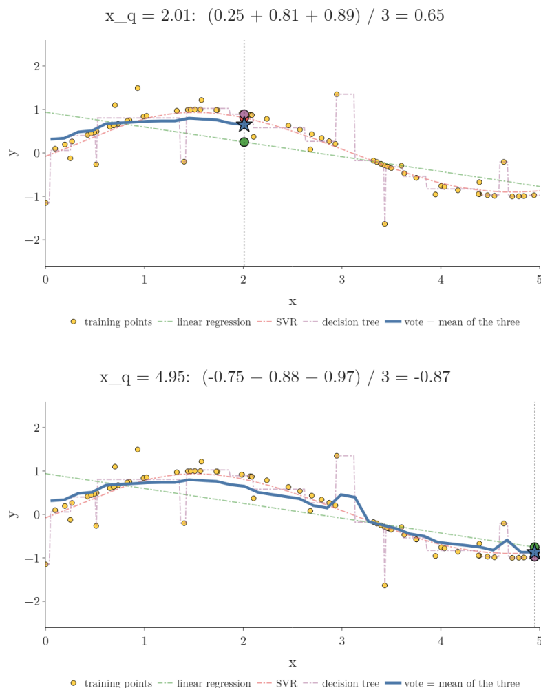
Figure 1: A query point sweeps across the sine data of section 3; at each position the three base regressors give a number each (coloured dots), and the vote is their mean (blue star)
