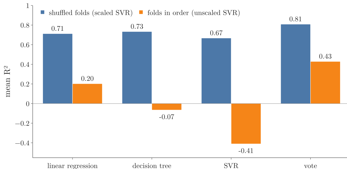
Figure 6: Mean R^2 with shuffled folds (blue) and with folds in order (orange), per model
