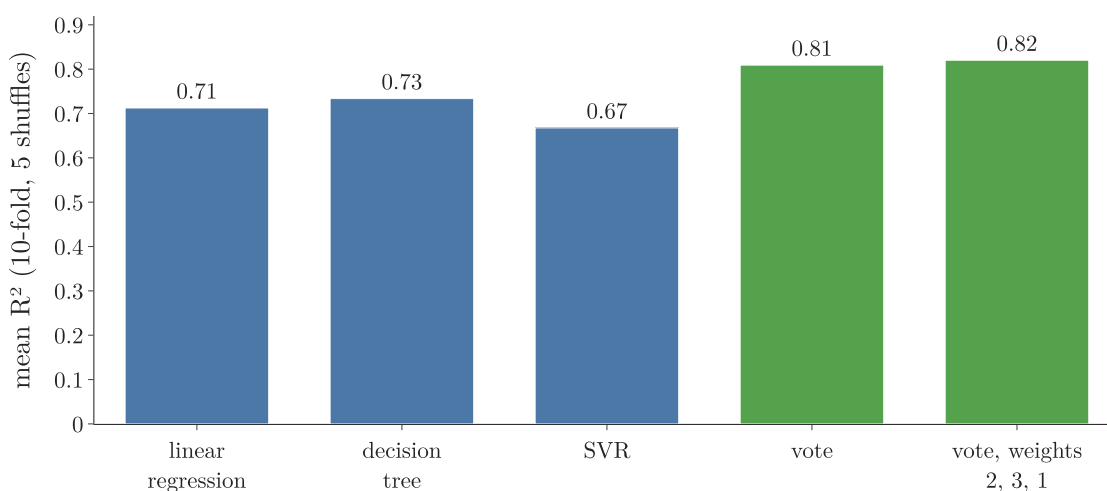
Figure 3: Mean R^2 on the Boston housing data: the three base models, their vote, and the vote with the best weights (2, 3, 1)
