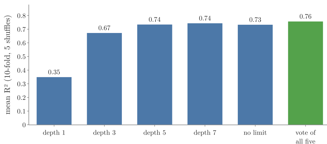
Figure 4: Mean R^2 of five decision trees of different depth on the Boston data, and of their vote
