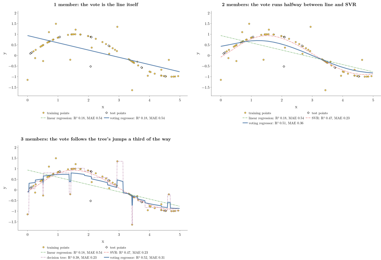
Figure 2: Base regressors (dash-dot) added one at a time on the noisy sine data, and the voting regressor (solid blue) after each addition: the line alone, then halfway between line and SVR, then the mean of line, SVR and tree. Legends give R^2 and MAE on the 8 test points
