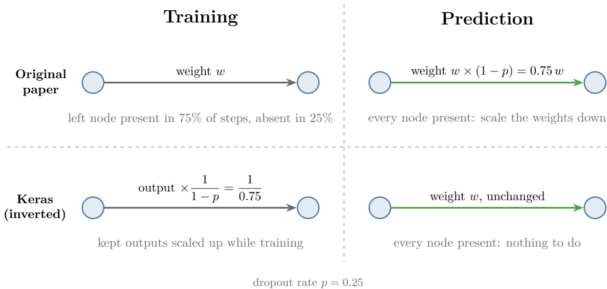
Figure 4: Two equivalent ways to handle dropout. Top: the original paper scales the weights down at prediction. Bottom: Keras scales the kept outputs up during training, so nothing changes at prediction.
