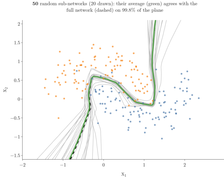
Figure 3: Sub-networks of one trained dropout network. Grey: the decision boundaries of single random sub-networks. Green: the boundary of their average output. Dashed black: the full network with every node, as used at prediction.
