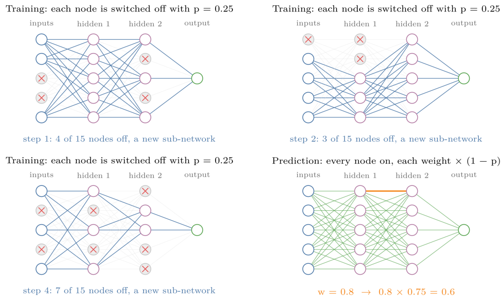
Figure 2: Dropout with p = 0.25 on the network of Figure 1, over four training steps. Each step draws a new random set of switched-off nodes (red crosses), and their connections go grey. At prediction every node is back, and each weight is multiplied by 1 - p = 0.75
