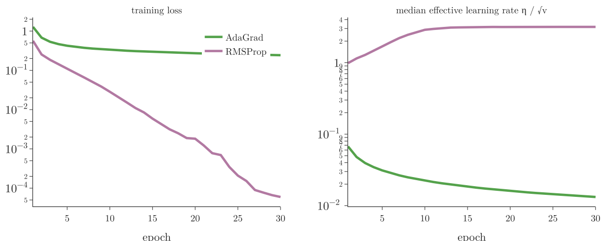
Figure 4: MNIST, mean of 3 seeds. Left: training loss per epoch. Right: the median effective learning rate. AdaGrad’s (green) falls epoch after epoch and its loss levels off; RMSProp’s (purple) does not fall, and its loss keeps dropping
