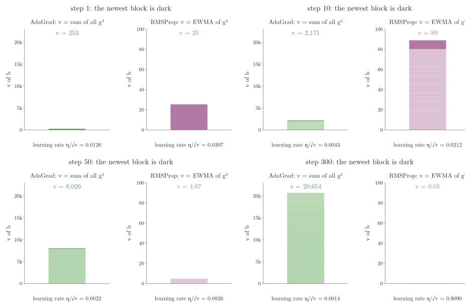
Figure 2: The accumulator v of the bias b drawn as a stack of blocks, one per step, learning rate 0.2. Left, AdaGrad: each squared gradient is added and kept. Right, RMSProp (section 4): each new block is (1 - \beta)g^2 and every older block shrinks by \beta = 0.9 at each step. Below each stack: the learning rate \eta/\sqrt{v}
