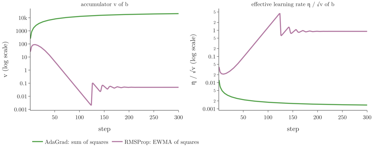
Figure 3: The accumulator v of the bias b and its effective learning rate \eta/\sqrt{v} , learning rate 0.2. AdaGrad's sum (green) only grows, so its learning rate only falls. RMSProp's average (purple) falls again as the gradients shrink near the minimum
