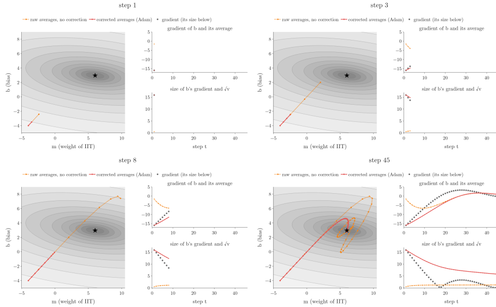
Figure 3: Adam, \eta = 0.5 , on the students data, step by step. Left: the path with corrected averages (red) and with the raw ones (dotted orange). Right, for the bias b of the red run: the gradient (grey dots) with m raw and corrected (top), and the gradient's size with \sqrt{v} raw and corrected (bottom)
