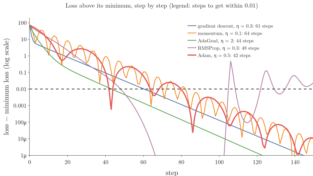
Figure 5: The loss above its minimum at every step for the five runs of the table, on a log scale. The dashed line is the 0.01 target; the legend gives the step at which each run first gets below it.
