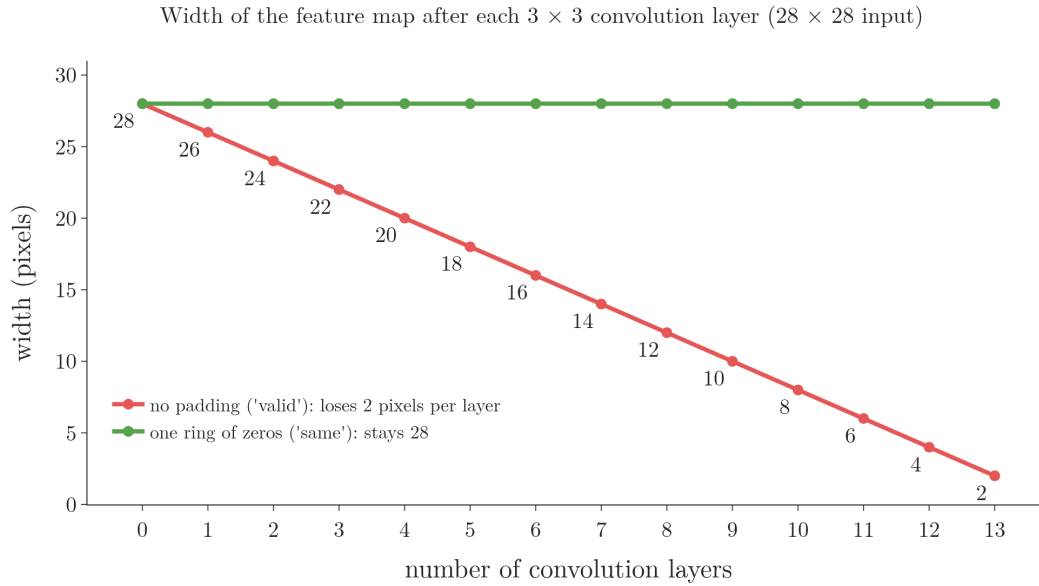
Figure 3: The width of the feature map after each 3 \times 3 convolution layer on a 28 \times 28 image, without padding (red) and with one ring of zeros (green). Sizes from Keras.
