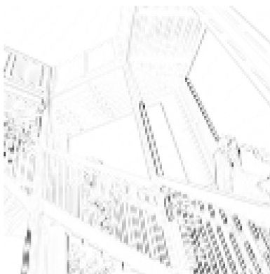
stride 2: 128 \times 128 map, 147,456 multiplications
