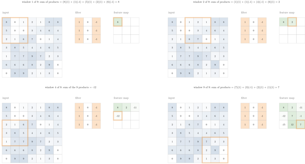
Figure 4: A 3 \times 3 filter on a 7 \times 7 image with stride 2: it jumps 2 pixels to the right and 2 pixels down, so it stops at only 3 \times 3 positions
