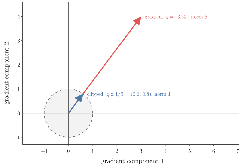
Figure 7: Clipping by norm with a threshold of 1. The gradient g = (3, 4) has norm 5, so it is multiplied by 1/5 : the clipped gradient (0.6, 0.8) points the same way and has norm 1
