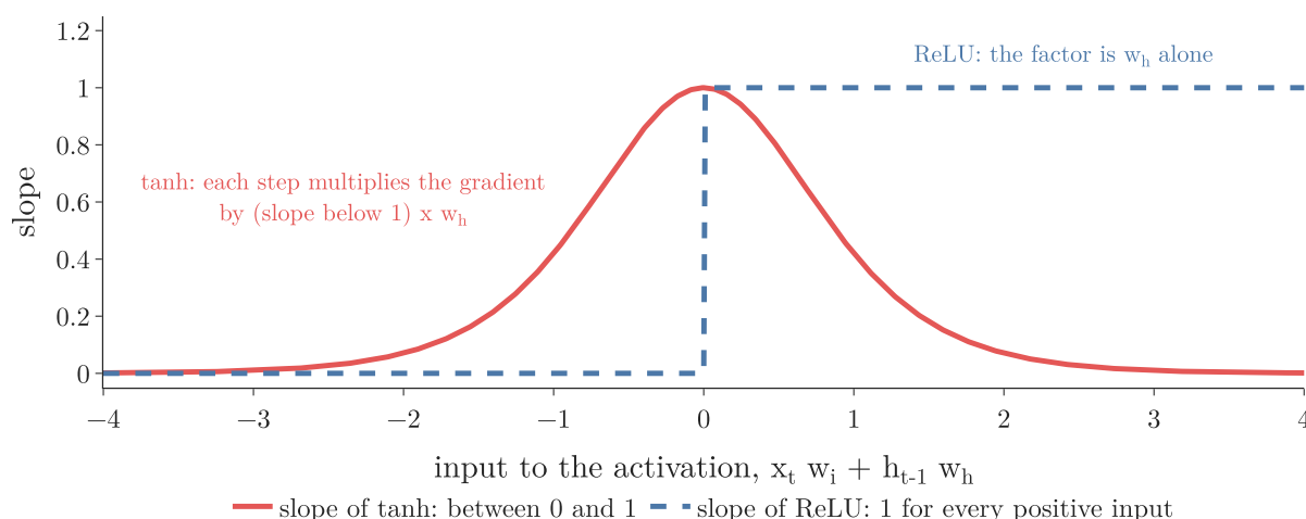
Figure 6: The slope of the activation, which multiplies w_h at every backward step. tanh’s slope (red) is 1 only at 0 and smaller everywhere else, so each step shrinks the gradient. ReLU’s slope (blue) is exactly 1 for every positive input, so the factor is w_h alone
