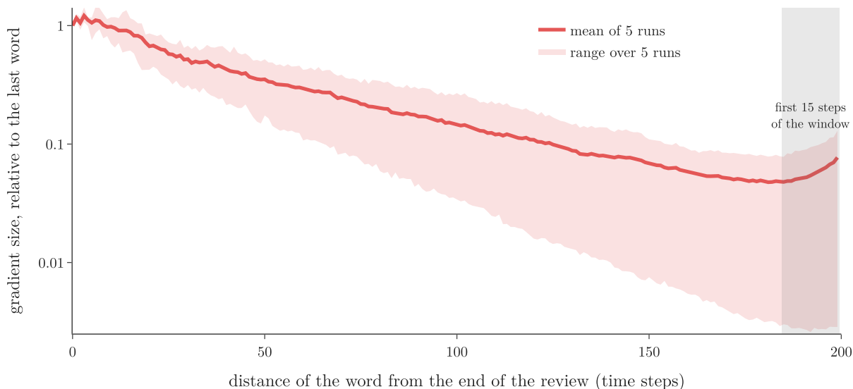
Figure 5: Gradient of the loss with respect to each word of a review, relative to the last word, for a SimpleRNN trained on IMDB (500 reviews of 200 words; red line: mean of 5 runs; band: range over the runs). Log scale. The grey strip marks the first 15 words of the 200-word window, explained at the end of this section
