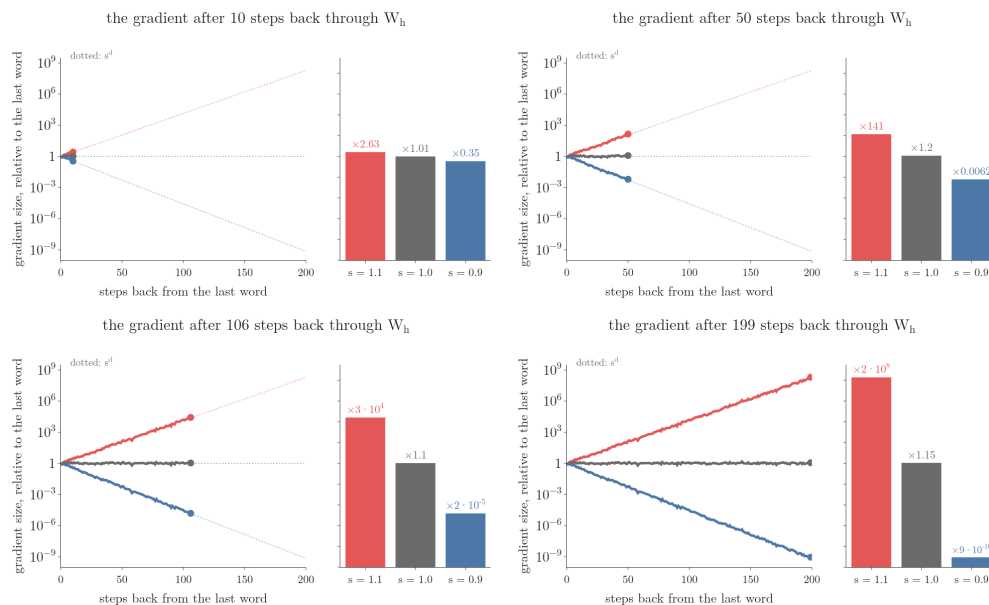
Figure 4: The gradient travelling back through an untrained SimpleRNN without activation on IMDB reviews, with W_h set to s times an orthogonal matrix (all eigenvalues of magnitude 1). Left: gradient size by distance, relative to the last word (log scale); dotted: s^d . Right: the size reached so far. Each step multiplies the gradient by about s
