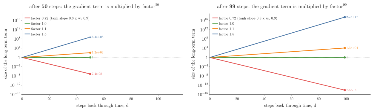
Figure 3: The same factor multiplied once per step back through time, for four factors (log scale). Below 1 the product falls towards 0 (vanishing); at 1 it stays; above 1 it grows without limit (exploding). The red line is the 0.72^{99} of section 4.3; the orange and blue lines are the two examples of section 6.1 (idea after StatQuest, “Recurrent Neural Networks (RNNs), Clearly Explained!!!”)
